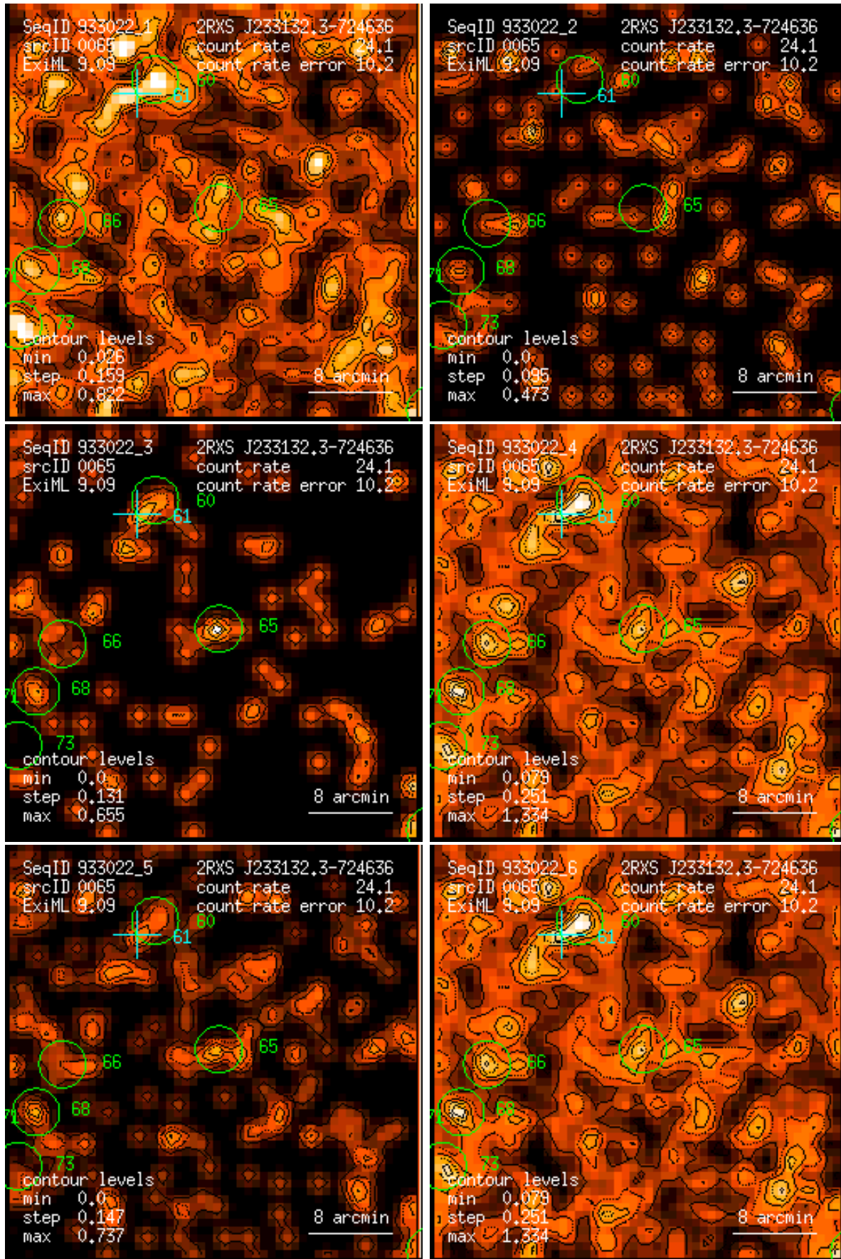
Figure 65: RASS 933022: detection 0065: band rate images, Gaussian filter: (1) PSPC channels 11 – 41, (2) 52 – 90, (3) 91 – 201, (4) 11 – 235, (5) 52 – 201, (6) 11 – 201. Broad band rates in counts/ks. Band rate contour levels in counts/ks/arcmin 2 .
