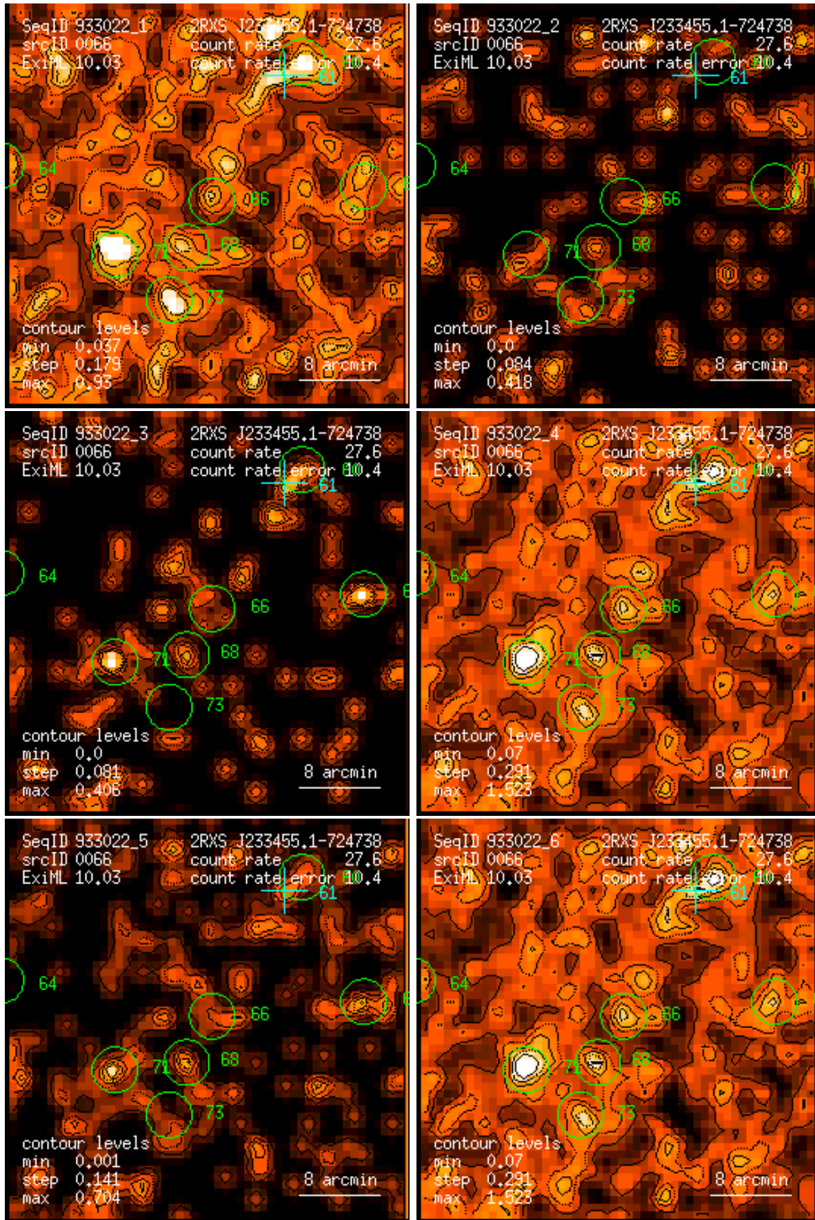
Figure 66: RASS 933022: detection 0066: band rate images, Gaussian filter: (1) PSPC channels 11 – 41, (2) 52 – 90, (3) 91 – 201, (4) 11 – 235, (5) 52 – 201, (6) 11 – 201. Broad band rates in counts/ks. Band rate contour levels in counts/ks/arcmin 2 .
