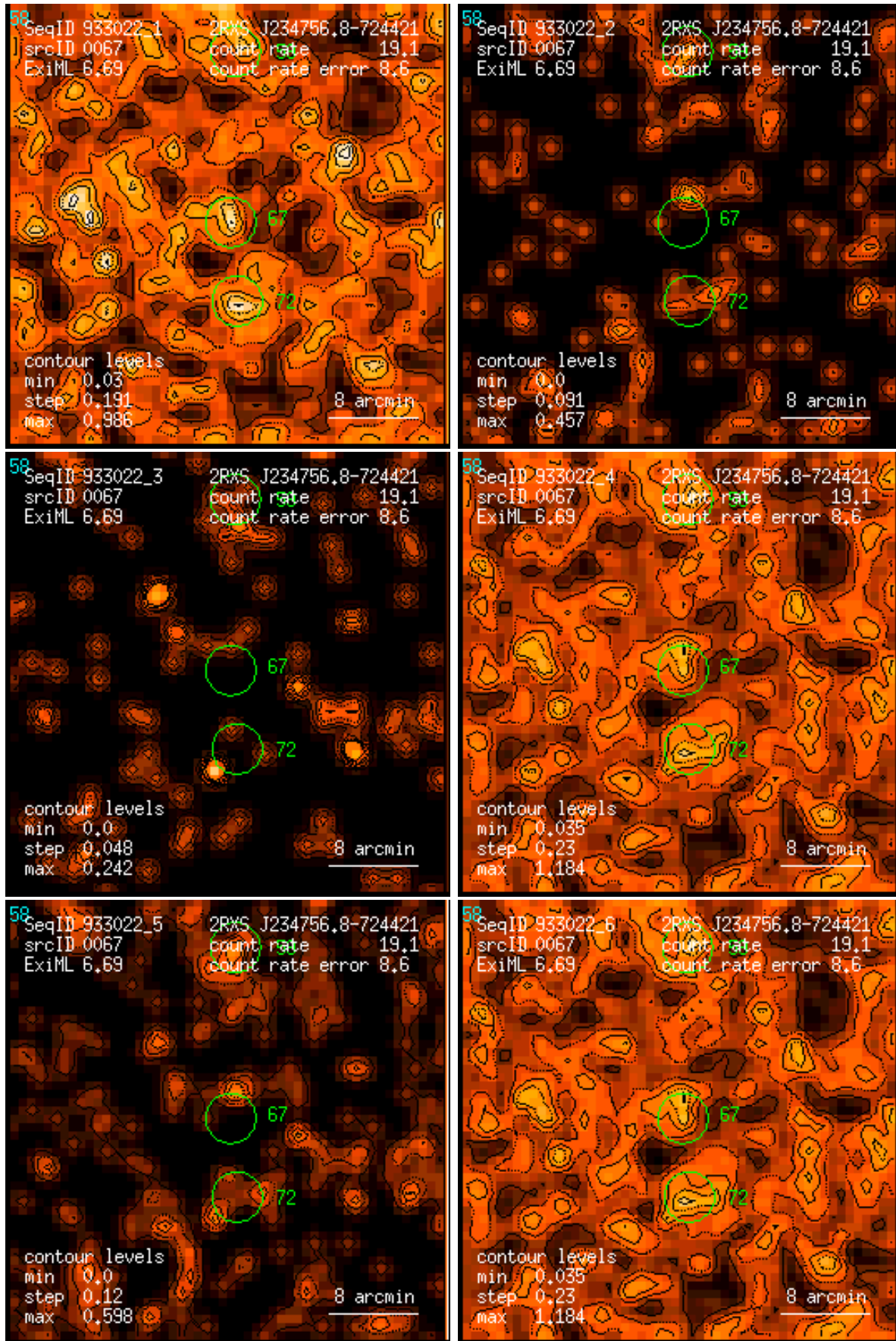
Figure 67: RASS 933022: detection 0067: band rate images, Gaussian filter: (1) PSPC channels 11 – 41, (2) 52 – 90, (3) 91 – 201, (4) 11 – 235, (5) 52 – 201, (6) 11 – 201. Broad band rates in counts/ks. Band rate contour levels in counts/ks/arcmin 2 .
