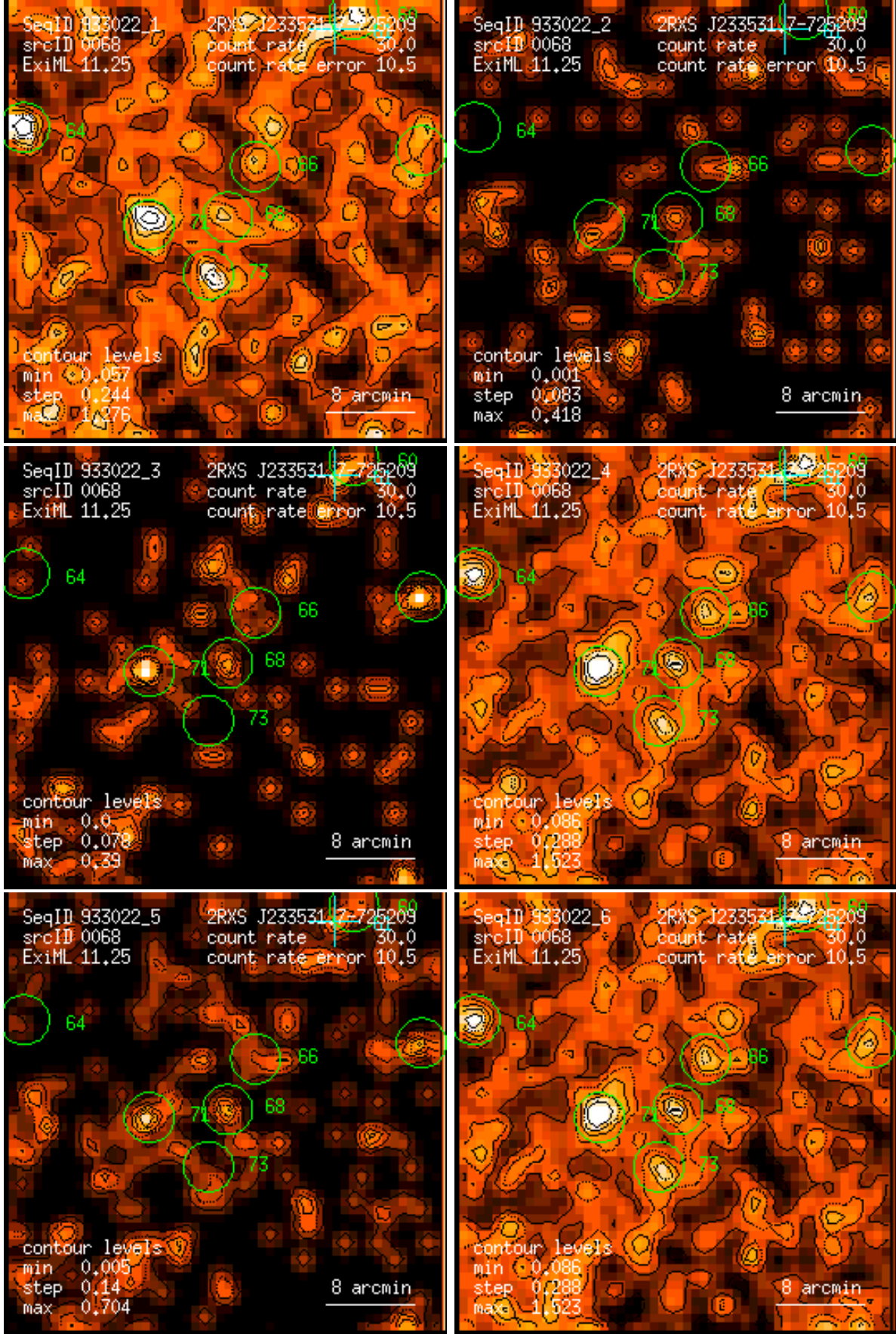
Figure 68: RASS 933022: detection 0068: band rate images, Gaussian filter: (1) PSPC channels 11 – 41, (2) 52 – 90, (3) 91 – 201, (4) 11 – 235, (5) 52 – 201, (6) 11 – 201. Broad band rates in counts/ks. Band rate contour levels in counts/ks/arcmin 2 .
