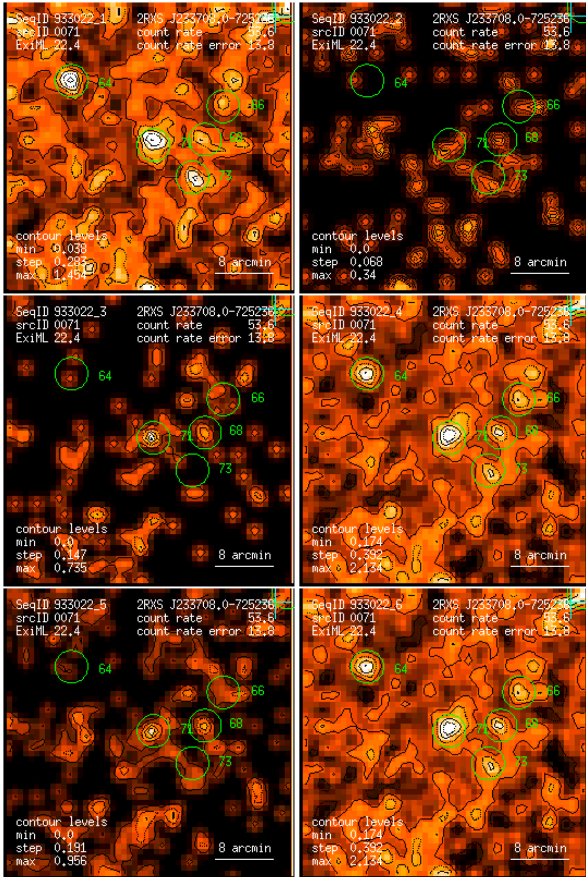
Figure 71: RASS 933022: detection 0071: band rate images, Gaussian filter: (1) PSPC channels 11 – 41, (2) 52 – 90, (3) 91 – 201, (4) 11 – 235, (5) 52 – 201, (6) 11 – 201. Broad band rates in counts/ks. Band rate contour levels in counts/ks/arcmin 2 .
