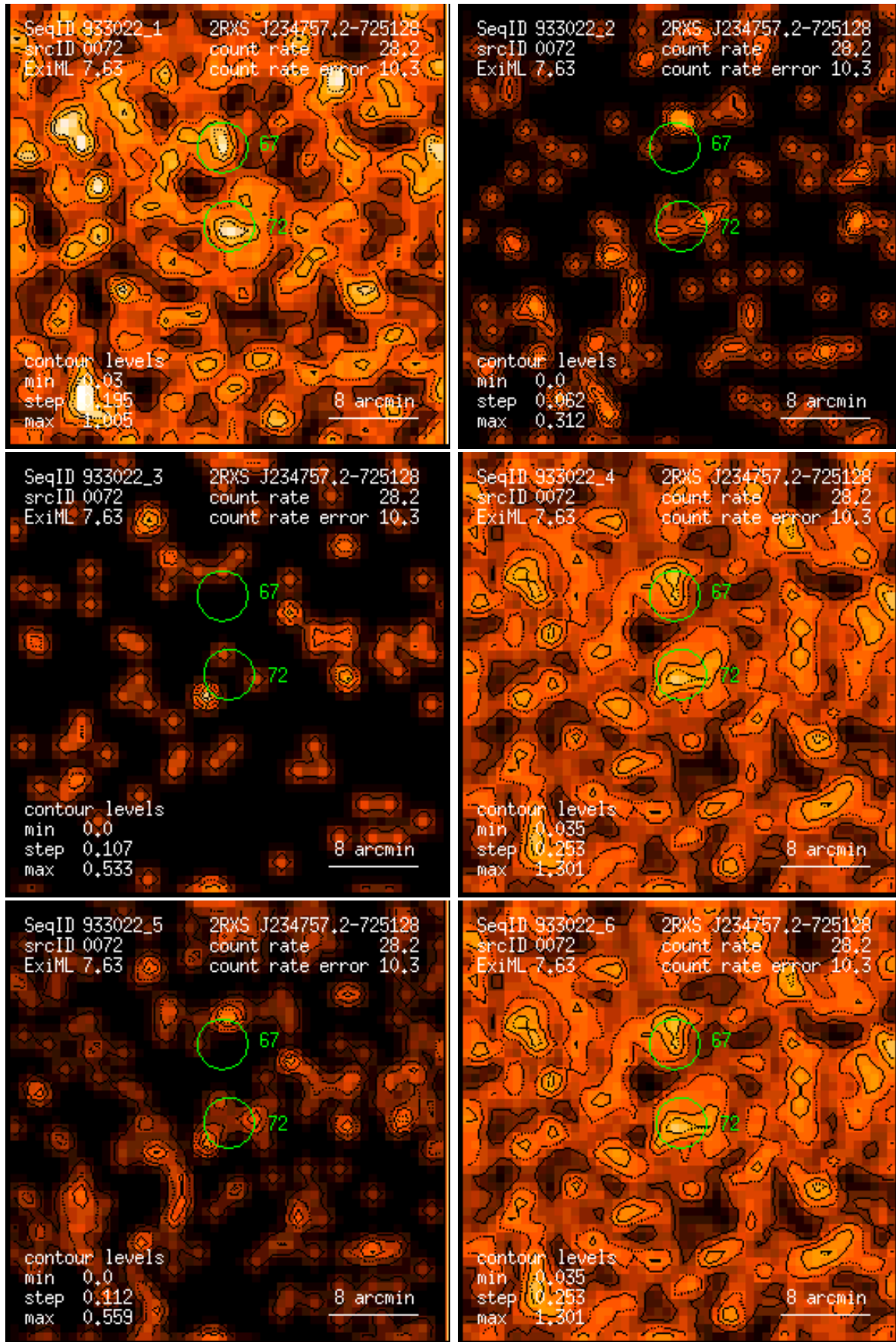
Figure 72: RASS 933022: detection 0072: band rate images, Gaussian filter: (1) PSPC channels 11 – 41, (2) 52 – 90, (3) 91 – 201, (4) 11 – 235, (5) 52 – 201, (6) 11 – 201. Broad band rates in counts/ks. Band rate contour levels in counts/ks/arcmin 2 .
