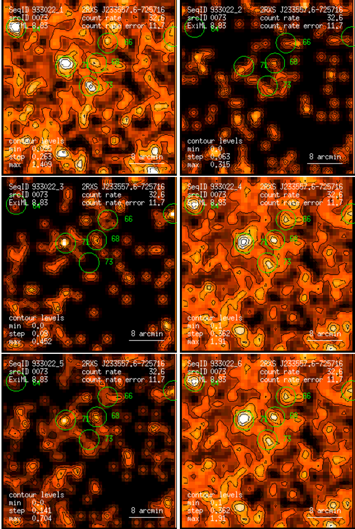
Figure 73: RASS 933022: detection 0073: band rate images, Gaussian filter: (1) PSPC channels 11 – 41, (2) 52 – 90, (3) 91 – 201, (4) 11 – 235, (5) 52 – 201, (6) 11 – 201. Broad band rates in counts/ks. Band rate contour levels in counts/ks/arcmin 2 .
