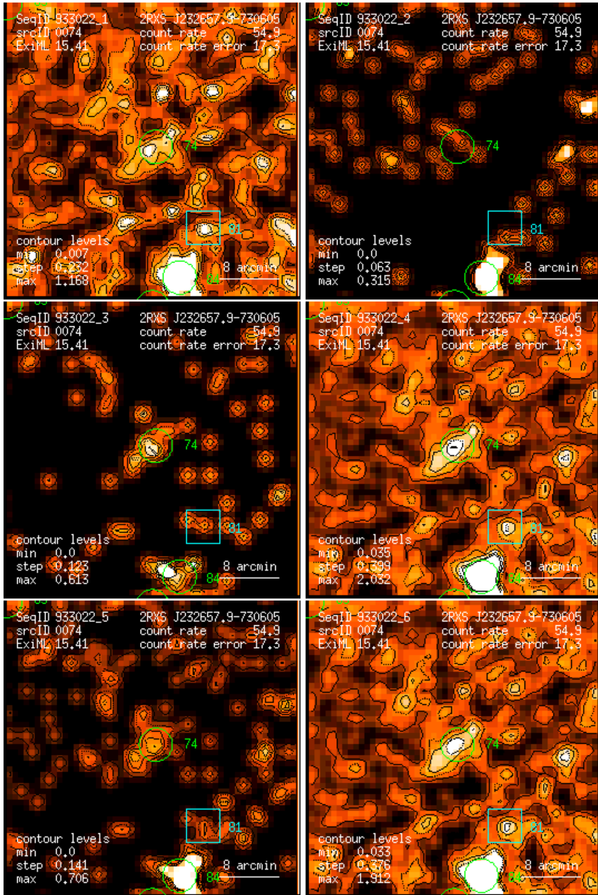
Figure 74: RASS 933022: detection 0074: band rate images, Gaussian filter: (1) PSPC channels 11 – 41, (2) 52 – 90, (3) 91 – 201, (4) 11 – 235, (5) 52 – 201, (6) 11 – 201. Broad band rates in counts/ks. Band rate contour levels in counts/ks/arcmin 2 .
