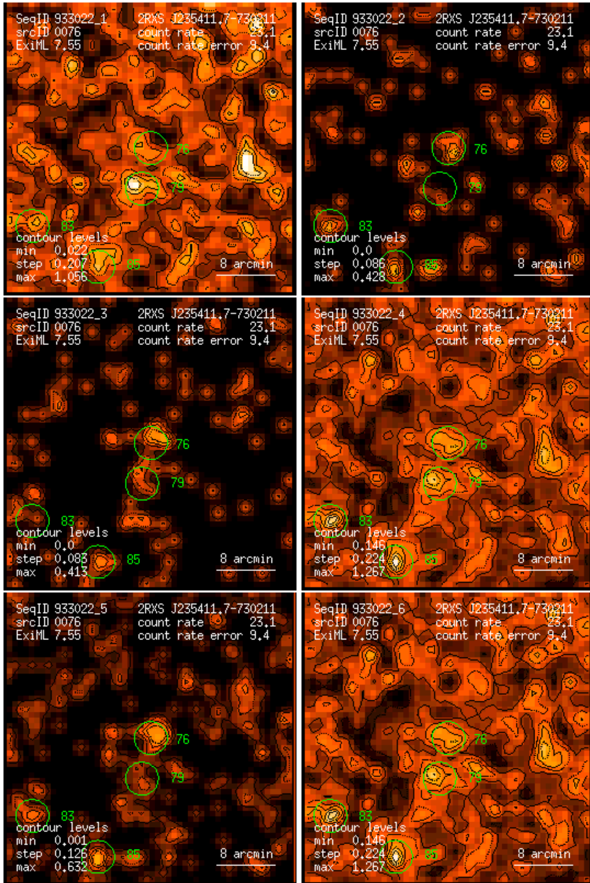
Figure 76: RASS 933022: detection 0076: band rate images, Gaussian filter: (1) PSPC channels 11 – 41, (2) 52 – 90, (3) 91 – 201, (4) 11 – 235, (5) 52 – 201, (6) 11 – 201. Broad band rates in counts/ks. Band rate contour levels in counts/ks/arcmin 2 .
