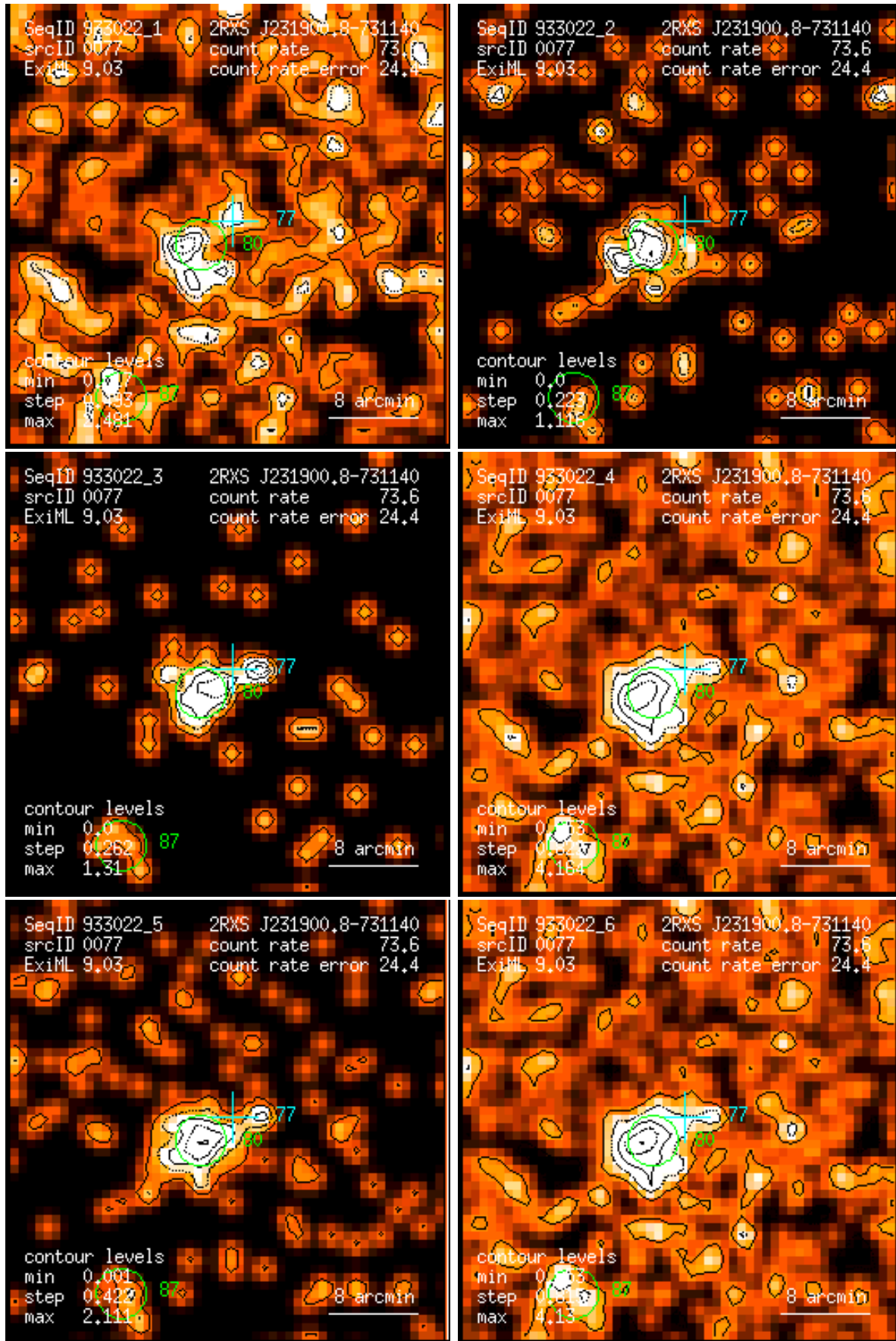
Figure 77: RASS 933022: detection 0077: band rate images, Gaussian filter: (1) PSPC channels 11 – 41, (2) 52 – 90, (3) 91 – 201, (4) 11 – 235, (5) 52 – 201, (6) 11 – 201. Broad band rates in counts/ks. Band rate contour levels in counts/ks/arcmin 2 .
