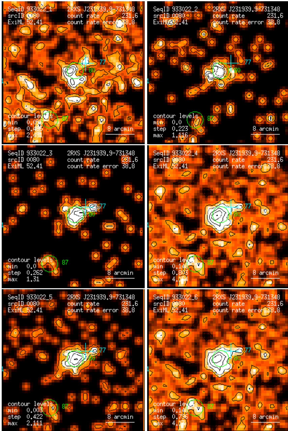
Figure 80: RASS 933022: detection 0080: band rate images, Gaussian filter: (1) PSPC channels 11 – 41, (2) 52 – 90, (3) 91 – 201, (4) 11 – 235, (5) 52 – 201, (6) 11 – 201. Broad band rates in counts/ks. Band rate contour levels in counts/ks/arcmin 2 .
