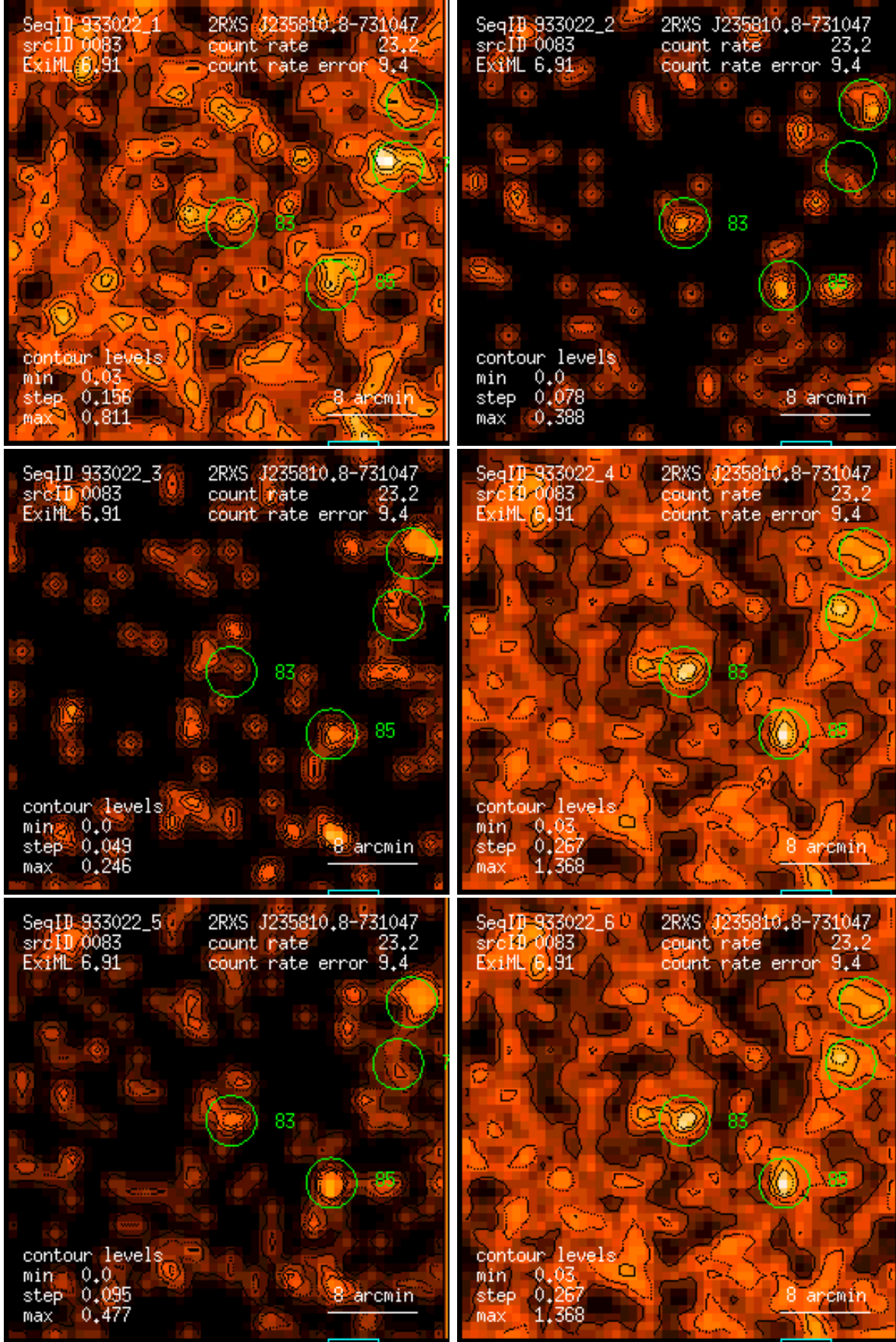
Figure 83: RASS 933022: detection 0083: band rate images, Gaussian filter: (1) PSPC channels 11 – 41, (2) 52 – 90, (3) 91 – 201, (4) 11 – 235, (5) 52 – 201, (6) 11 – 201. Broad band rates in counts/ks. Band rate contour levels in counts/ks/arcmin 2 .
