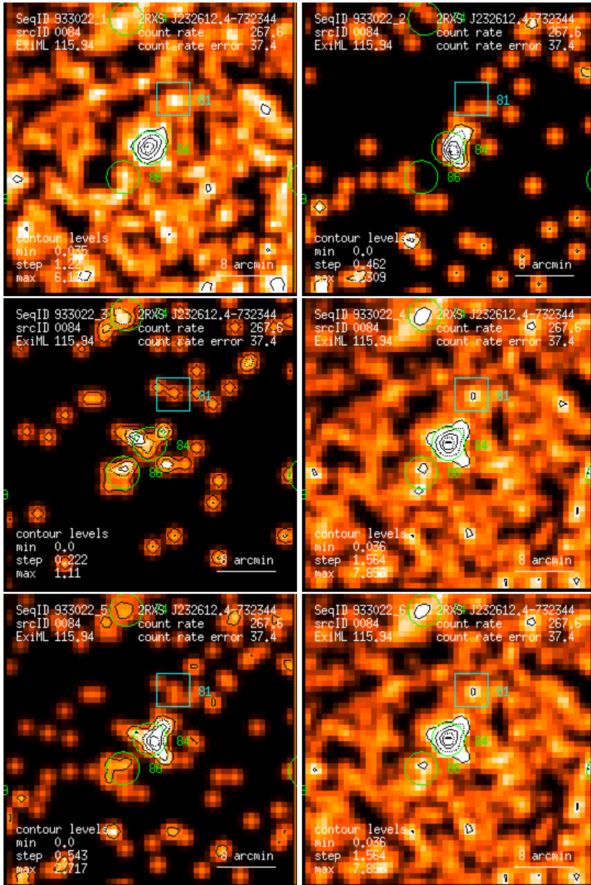
Figure 84: RASS 933022: detection 0084: band rate images, Gaussian filter: (1) PSPC channels 11 – 41, (2) 52 – 90, (3) 91 – 201, (4) 11 – 235, (5) 52 – 201, (6) 11 – 201. Broad band rates in counts/ks. Band rate contour levels in counts/ks/arcmin 2 .
