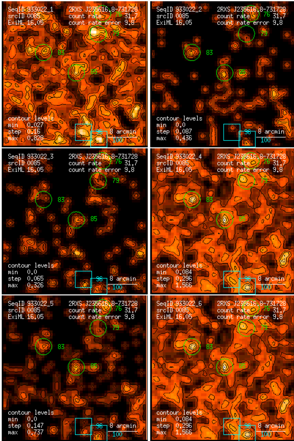
Figure 85: RASS 933022: detection 0085: band rate images, Gaussian filter: (1) PSPC channels 11 – 41, (2) 52 – 90, (3) 91 – 201, (4) 11 – 235, (5) 52 – 201, (6) 11 – 201. Broad band rates in counts/ks. Band rate contour levels in counts/ks/arcmin 2 .
