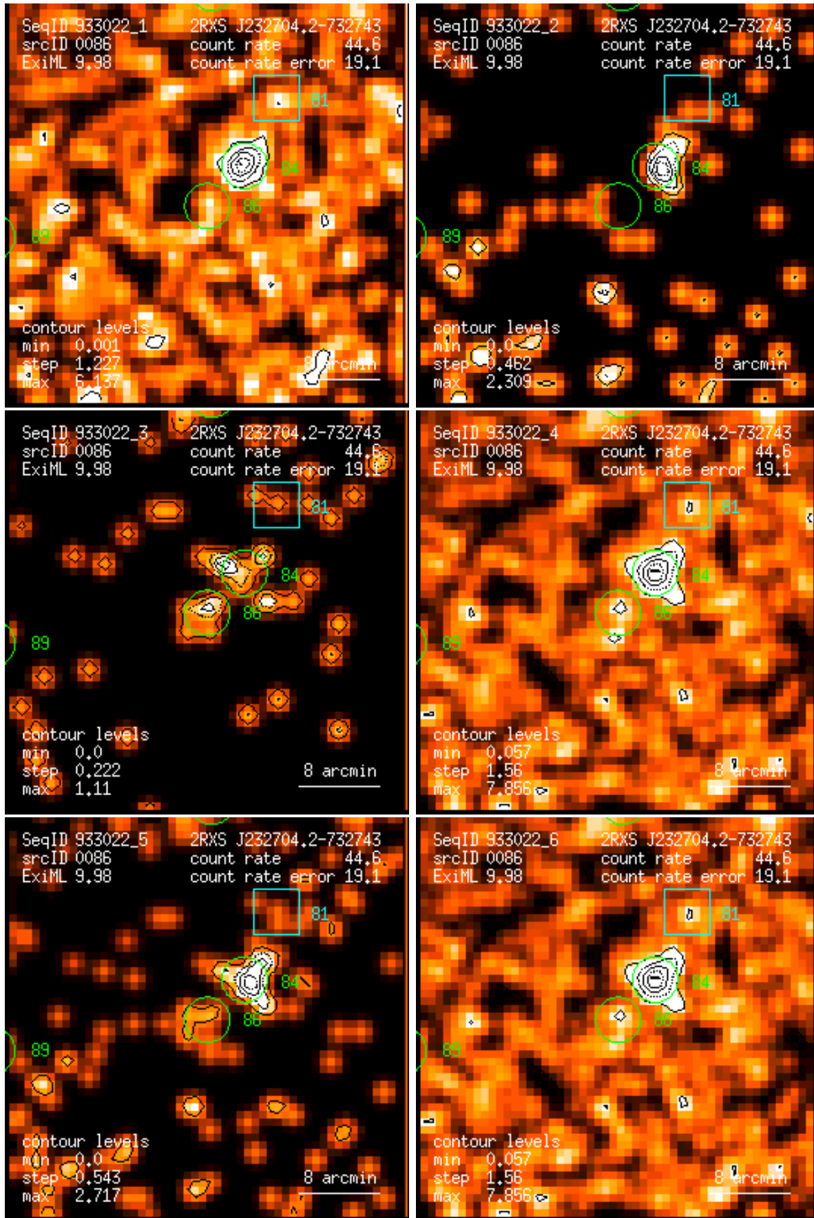
Figure 86: RASS 933022: detection 0086: band rate images, Gaussian filter: (1) PSPC channels 11 – 41, (2) 52 – 90, (3) 91 – 201, (4) 11 – 235, (5) 52 – 201, (6) 11 – 201. Broad band rates in counts/ks. Band rate contour levels in counts/ks/arcmin 2 .
