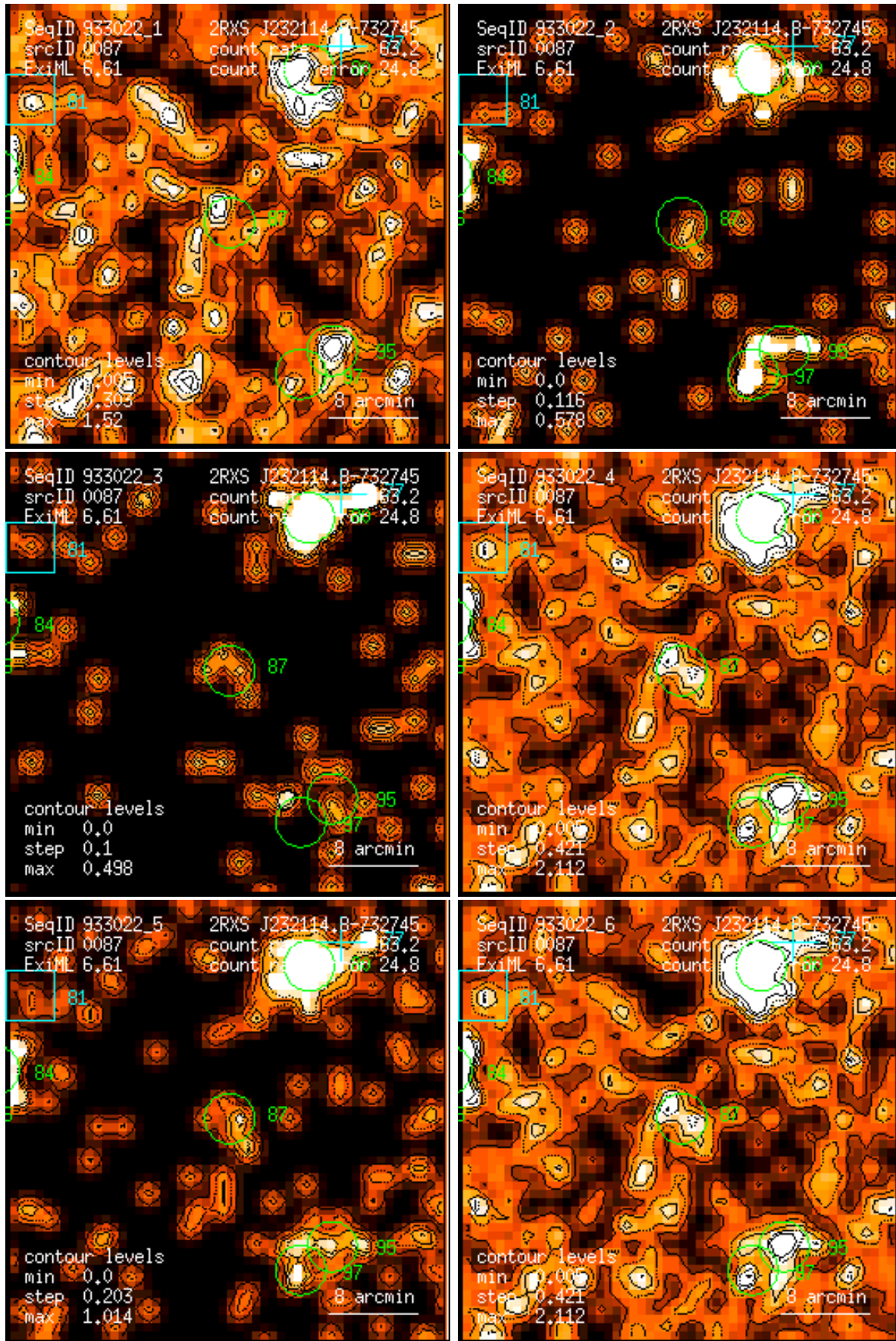
Figure 87: RASS 933022: detection 0087: band rate images, Gaussian filter: (1) PSPC channels 11 – 41, (2) 52 – 90, (3) 91 – 201, (4) 11 – 235, (5) 52 – 201, (6) 11 – 201. Broad band rates in counts/ks. Band rate contour levels in counts/ks/arcmin 2 .
