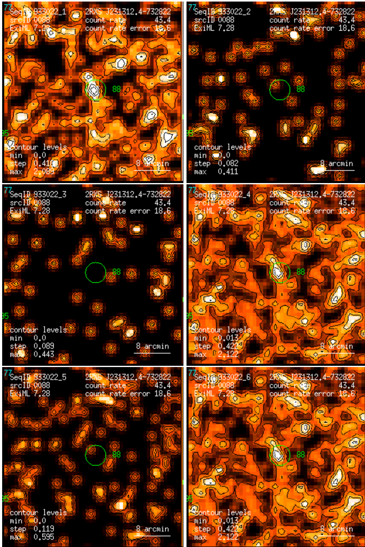
Figure 88: RASS 933022: detection 0088: band rate images, Gaussian filter: (1) PSPC channels 11 – 41, (2) 52 – 90, (3) 91 – 201, (4) 11 – 235, (5) 52 – 201, (6) 11 – 201. Broad band rates in counts/ks. Band rate contour levels in counts/ks/arcmin 2 .
