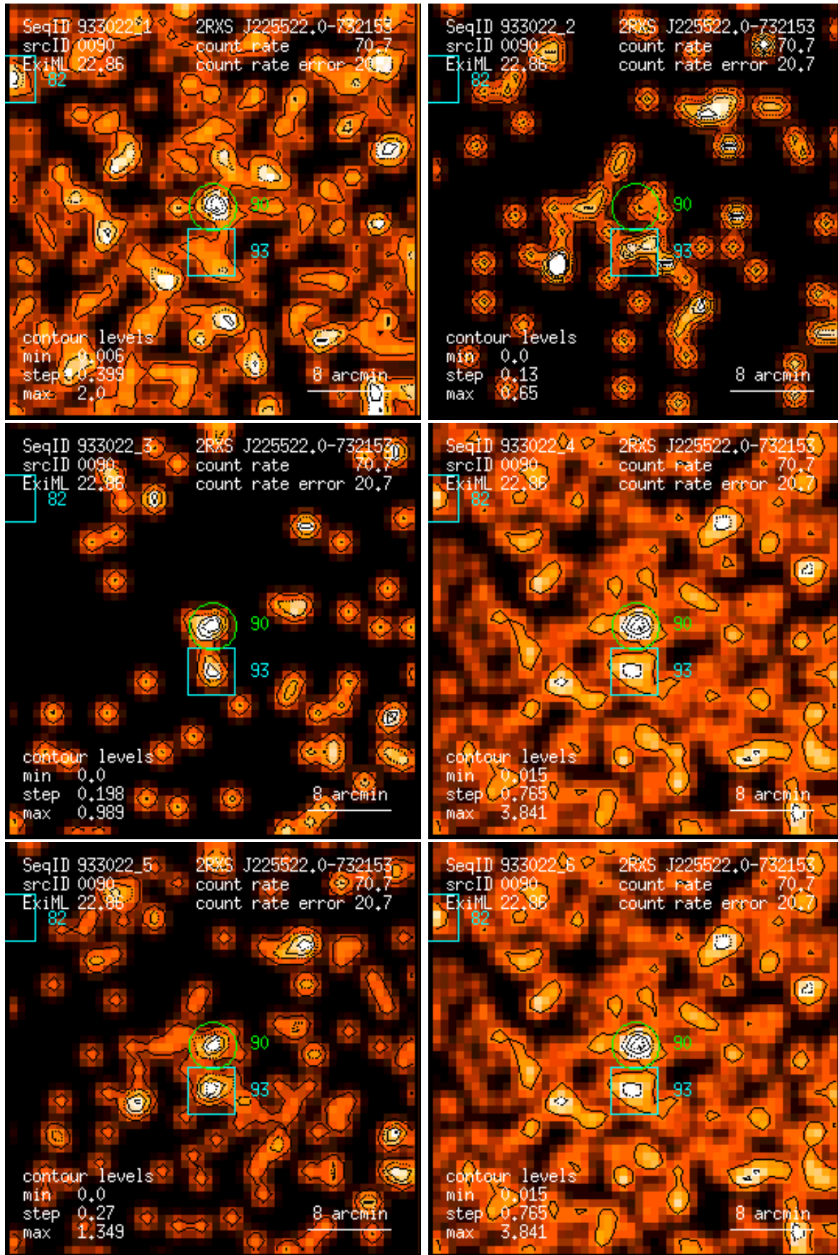
Figure 90: RASS 933022: detection 0090: band rate images, Gaussian filter: (1) PSPC channels 11 – 41, (2) 52 – 90, (3) 91 – 201, (4) 11 – 235, (5) 52 – 201, (6) 11 – 201. Broad band rates in counts/ks. Band rate contour levels in counts/ks/arcmin 2 .
