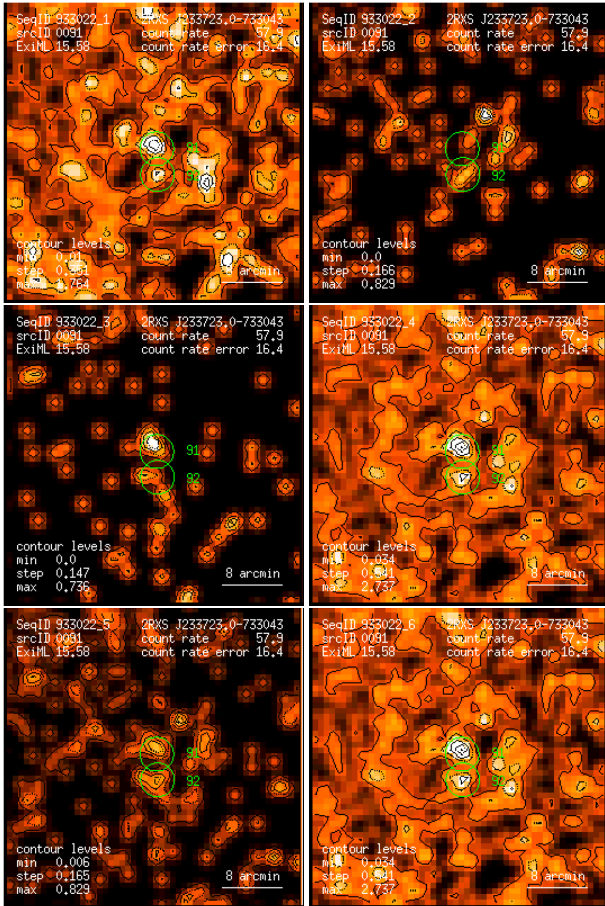
Figure 91: RASS 933022: detection 0091: band rate images, Gaussian filter: (1) PSPC channels 11 – 41, (2) 52 – 90, (3) 91 – 201, (4) 11 – 235, (5) 52 – 201, (6) 11 – 201. Broad band rates in counts/ks. Band rate contour levels in counts/ks/arcmin 2 .
