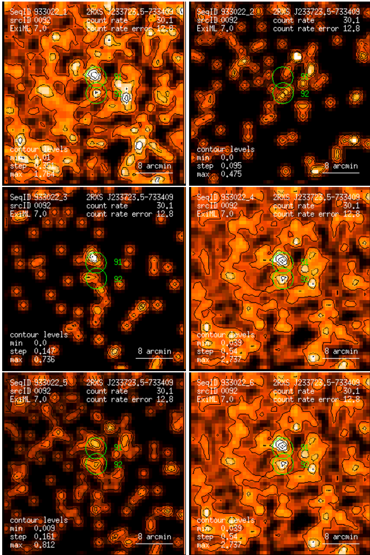
Figure 92: RASS 933022: detection 0092: band rate images, Gaussian filter: (1) PSPC channels 11 – 41, (2) 52 – 90, (3) 91 – 201, (4) 11 – 235, (5) 52 – 201, (6) 11 – 201. Broad band rates in counts/ks. Band rate contour levels in counts/ks/arcmin 2 .
