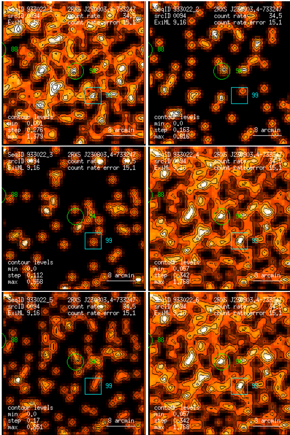
Figure 94: RASS 933022: detection 0094: band rate images, Gaussian filter: (1) PSPC channels 11 – 41, (2) 52 – 90, (3) 91 – 201, (4) 11 – 235, (5) 52 – 201, (6) 11 – 201. Broad band rates in counts/ks. Band rate contour levels in counts/ks/arcmin 2 .
