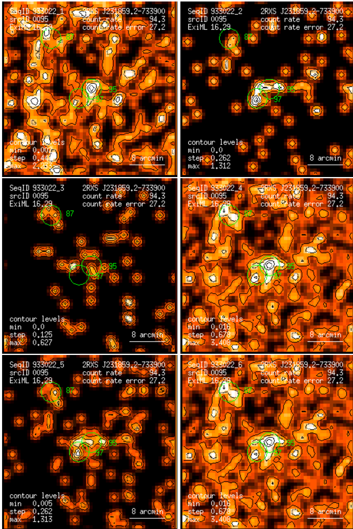
Figure 95: RASS 933022: detection 0095: band rate images, Gaussian filter: (1) PSPC channels 11 – 41, (2) 52 – 90, (3) 91 – 201, (4) 11 – 235, (5) 52 – 201, (6) 11 – 201. Broad band rates in counts/ks. Band rate contour levels in counts/ks/arcmin 2 .
