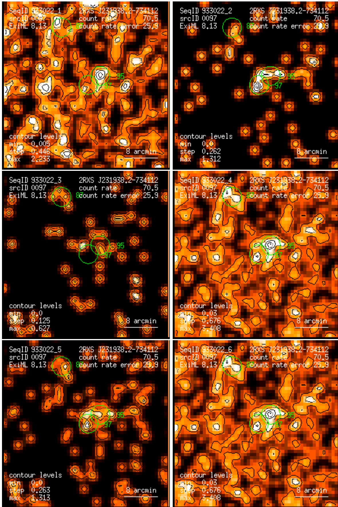
Figure 97: RASS 933022: detection 0097: band rate images, Gaussian filter: (1) PSPC channels 11 – 41, (2) 52 – 90, (3) 91 – 201, (4) 11 – 235, (5) 52 – 201, (6) 11 – 201. Broad band rates in counts/ks. Band rate contour levels in counts/ks/arcmin 2 .
