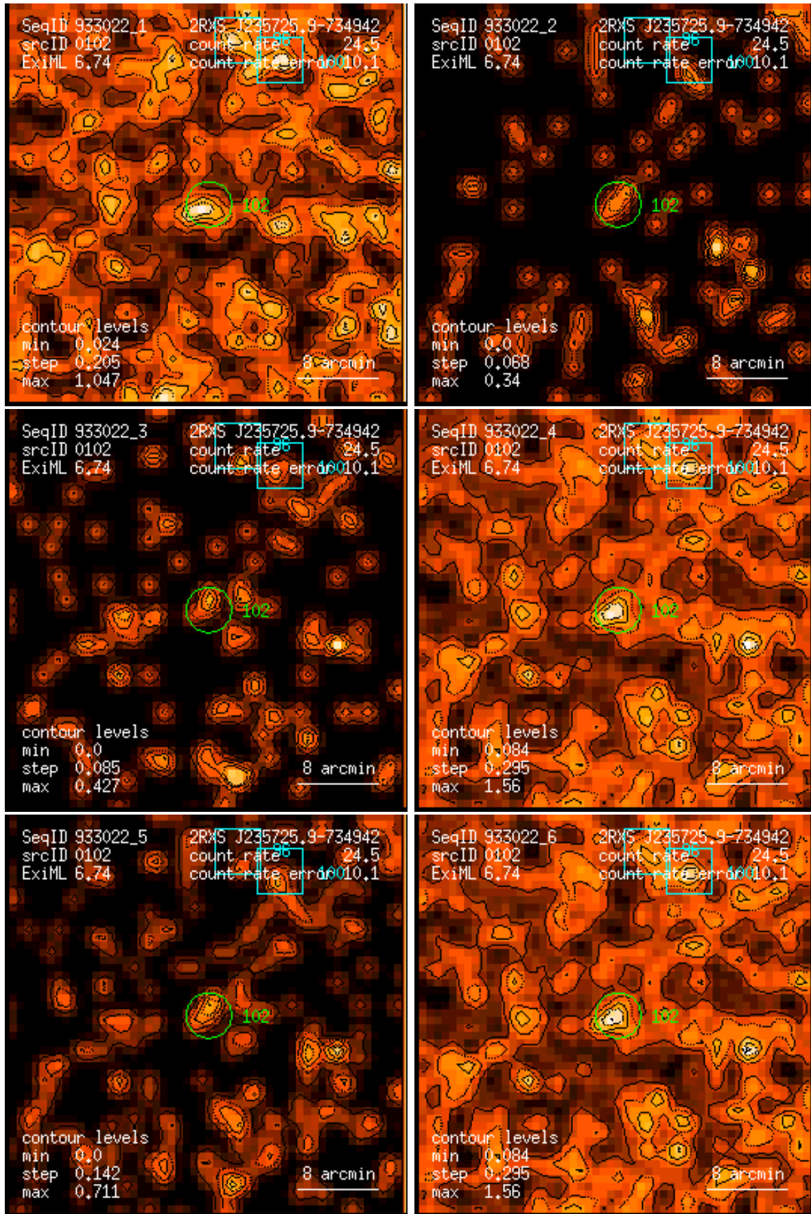
Figure 102: RASS 933022: detection 0102: band rate images, Gaussian filter: (1) PSPC channels 11 – 41, (2) 52 – 90, (3) 91 – 201, (4) 11 – 235, (5) 52 – 201, (6) 11 – 201. Broad band rates in counts/ks. Band rate contour levels in counts/ks/arcmin 2 .
