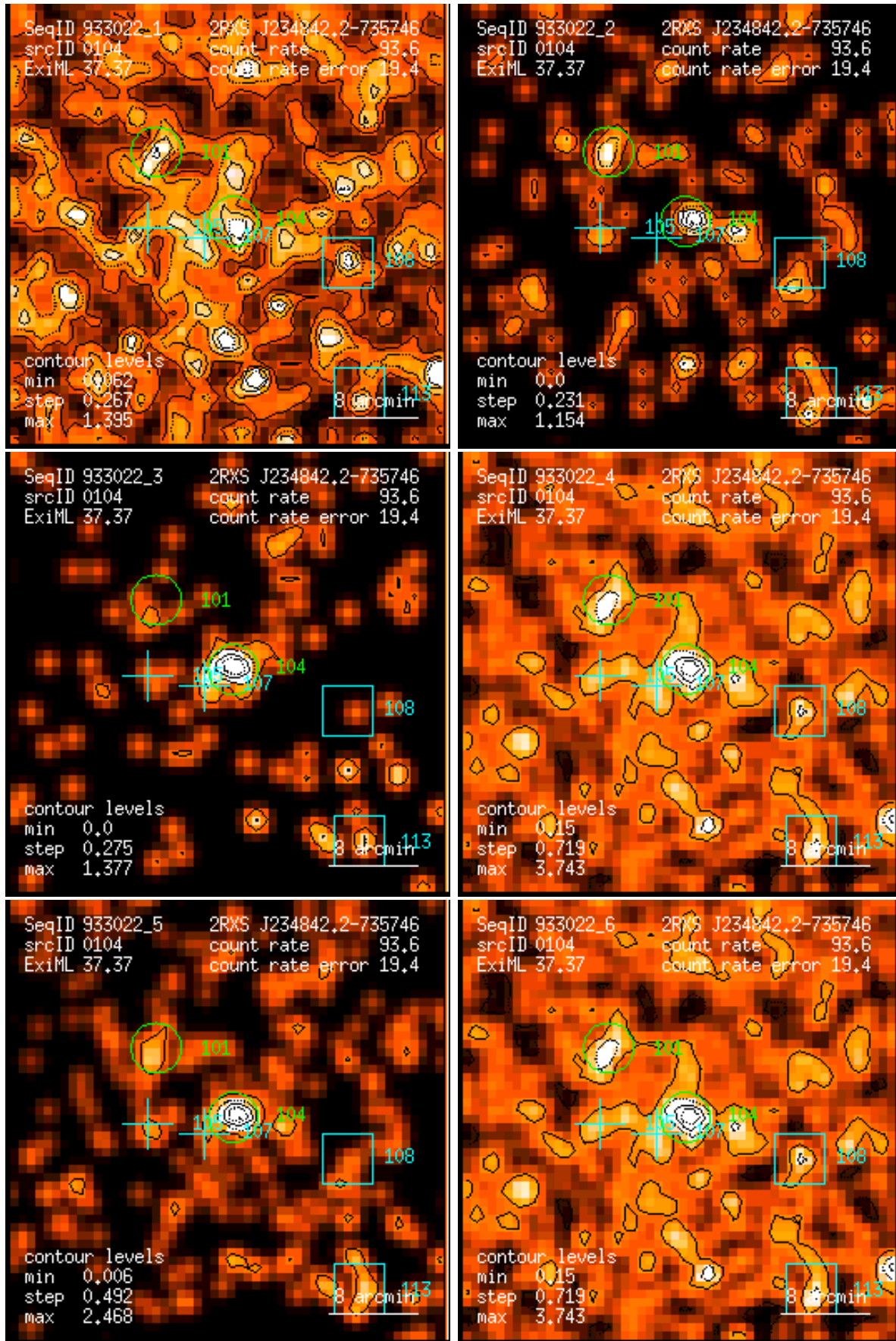
Figure 104: RASS 933022: detection 0104: band rate images, Gaussian filter: (1) PSPC channels 11 – 41, (2) 52 – 90, (3) 91 – 201, (4) 11 – 235, (5) 52 – 201, (6) 11 – 201. Broad band rates in counts/ks. Band rate contour levels in counts/ks/arcmin 2 .
