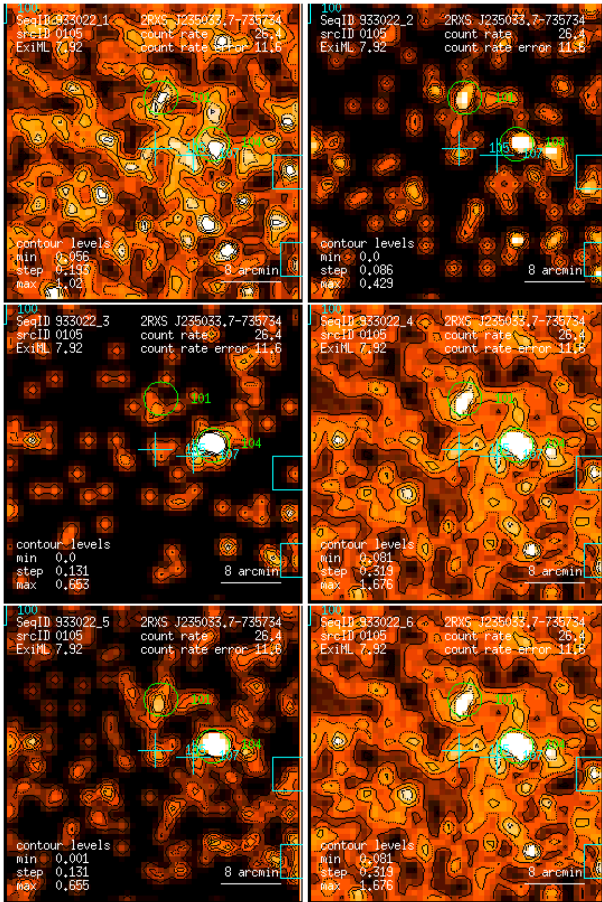
Figure 105: RASS 933022: detection 0105: band rate images, Gaussian filter: (1) PSPC channels 11 – 41, (2) 52 – 90, (3) 91 – 201, (4) 11 – 235, (5) 52 – 201, (6) 11 – 201. Broad band rates in counts/ks. Band rate contour levels in counts/ks/arcmin 2 .
