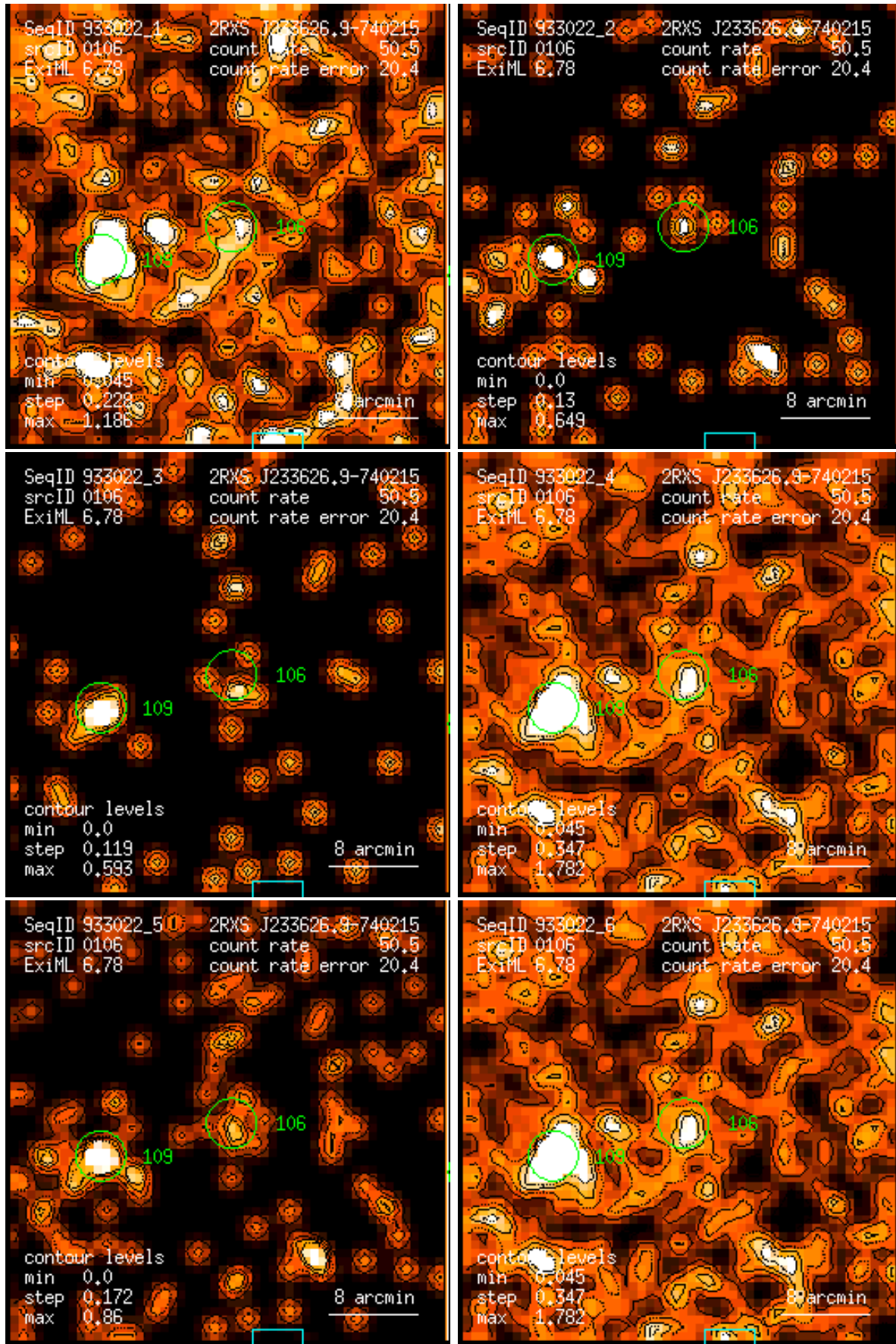
Figure 106: RASS 933022: detection 0106: band rate images, Gaussian filter: (1) PSPC channels 11 – 41, (2) 52 – 90, (3) 91 – 201, (4) 11 – 235, (5) 52 – 201, (6) 11 – 201. Broad band rates in counts/ks. Band rate contour levels in counts/ks/arcmin 2 .
