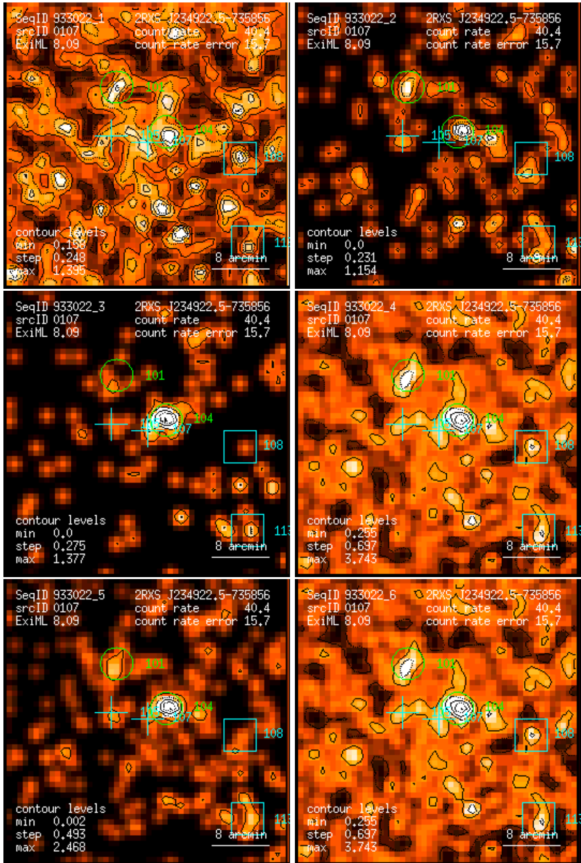
Figure 107: RASS 933022: detection 0107: band rate images, Gaussian filter: (1) PSPC channels 11 – 41, (2) 52 – 90, (3) 91 – 201, (4) 11 – 235, (5) 52 – 201, (6) 11 – 201. Broad band rates in counts/ks. Band rate contour levels in counts/ks/arcmin 2 .
