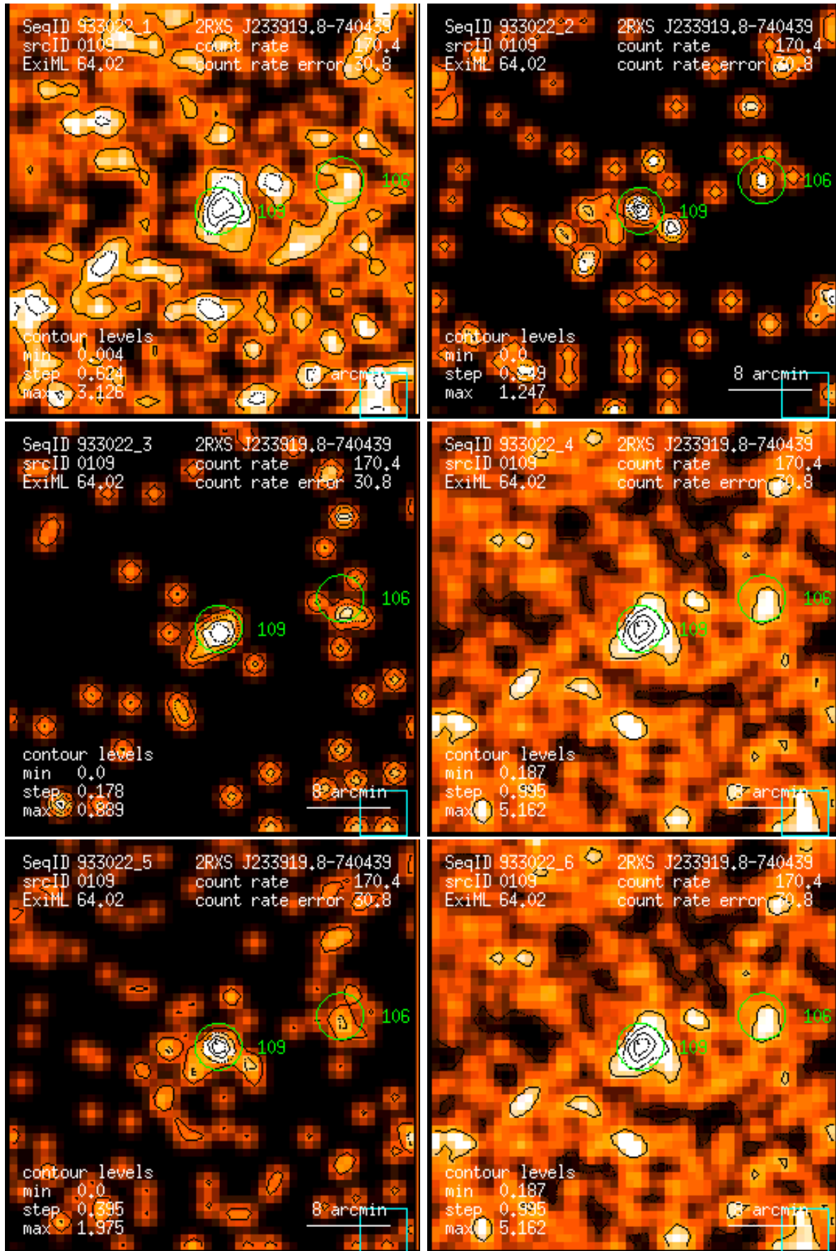
Figure 109: RASS 933022: detection 0109: band rate images, Gaussian filter: (1) PSPC channels 11 – 41, (2) 52 – 90, (3) 91 – 201, (4) 11 – 235, (5) 52 – 201, (6) 11 – 201. Broad band rates in counts/ks. Band rate contour levels in counts/ks/arcmin 2 .
