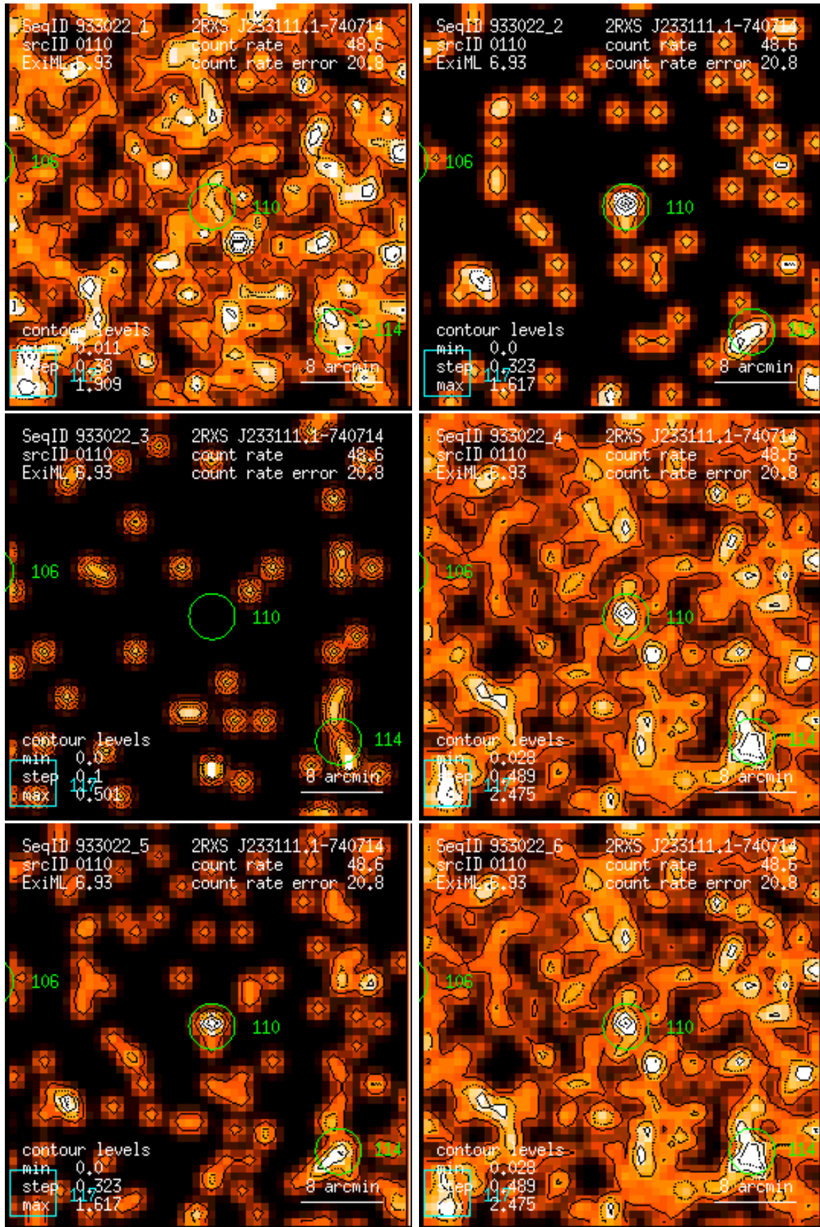
Figure 110: RASS 933022: detection 0110: band rate images, Gaussian filter: (1) PSPC channels 11 – 41, (2) 52 – 90, (3) 91 – 201, (4) 11 – 235, (5) 52 – 201, (6) 11 – 201. Broad band rates in counts/ks. Band rate contour levels in counts/ks/arcmin 2 .
