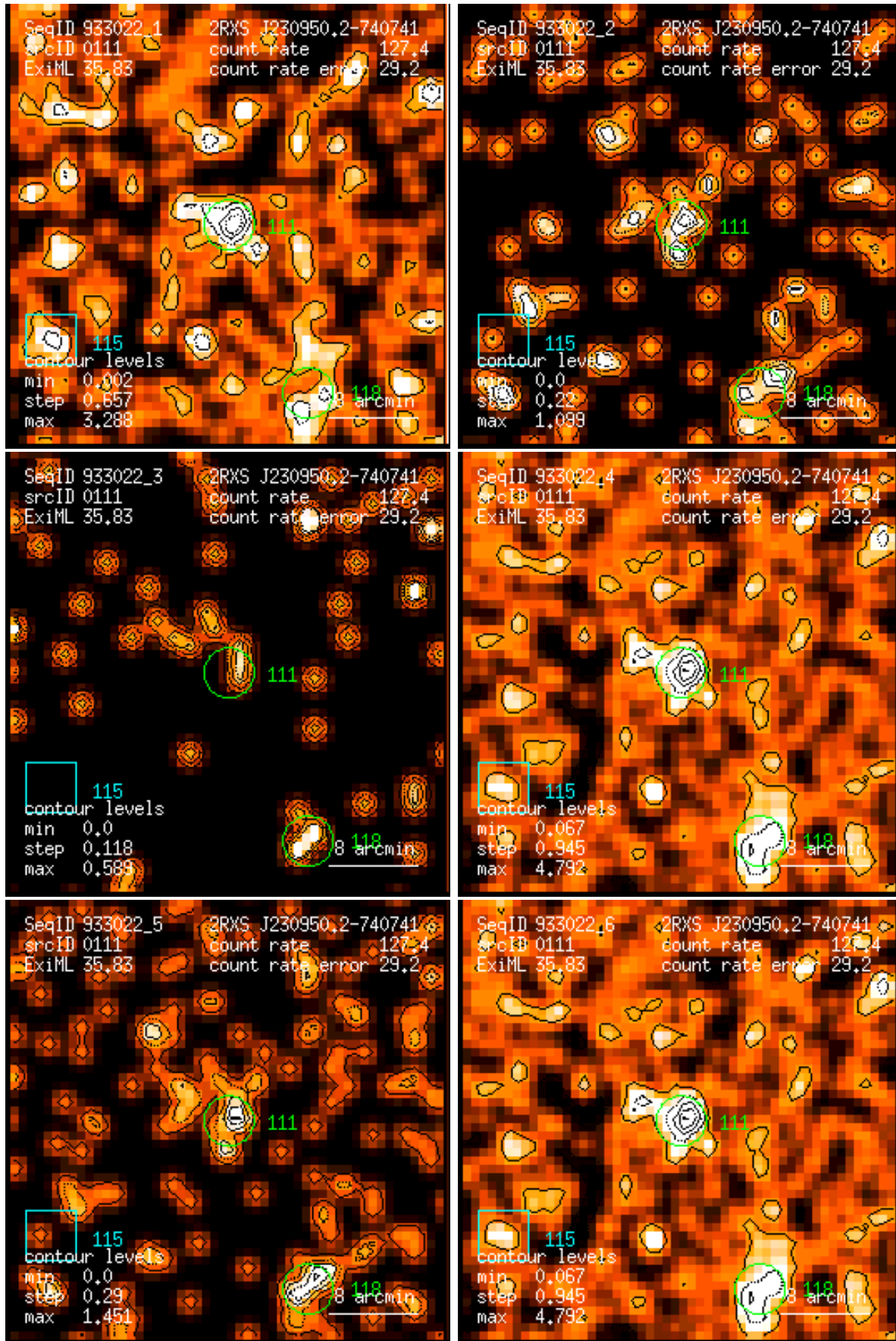
Figure 111: RASS 933022: detection 0111: band rate images, Gaussian filter: (1) PSPC channels 11 – 41, (2) 52 – 90, (3) 91 – 201, (4) 11 – 235, (5) 52 – 201, (6) 11 – 201. Broad band rates in counts/ks. Band rate contour levels in counts/ks/arcmin 2 .
