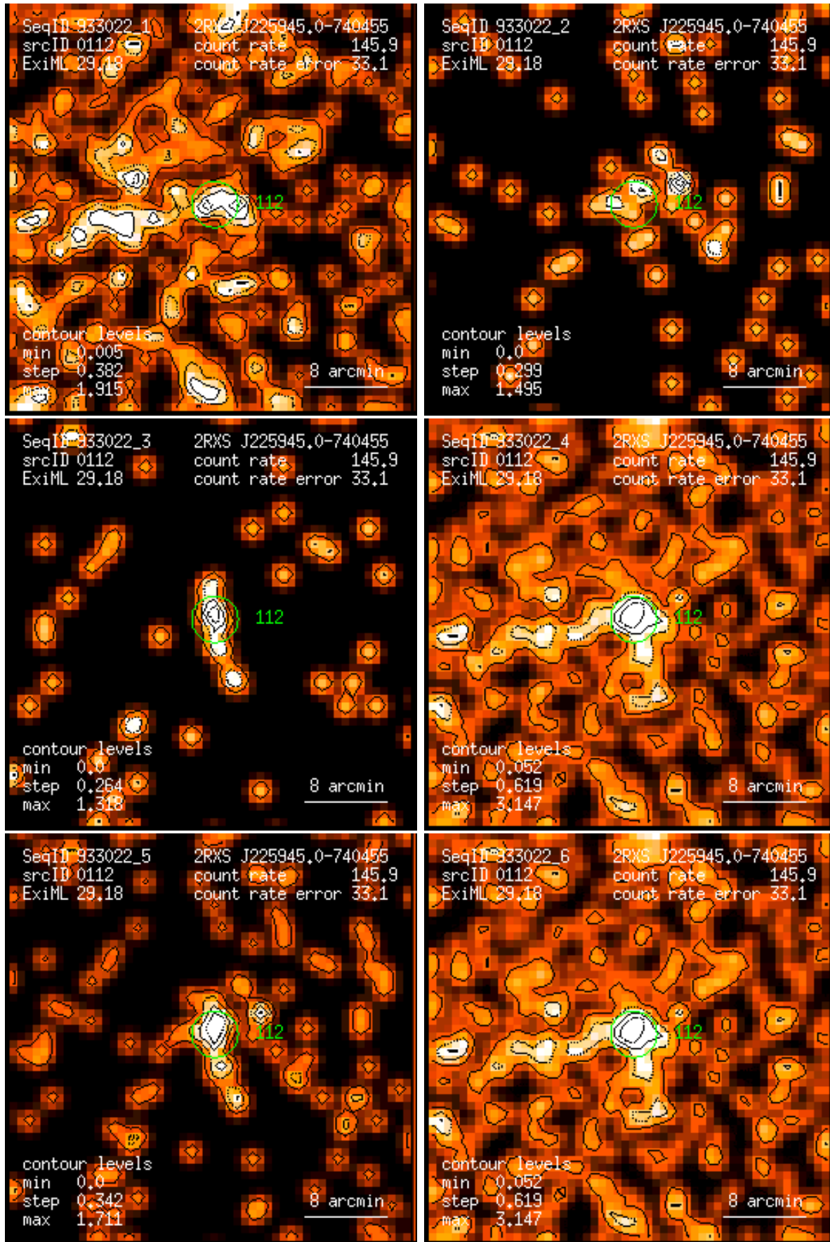
Figure 112: RASS 933022: detection 0112: band rate images, Gaussian filter: (1) PSPC channels 11 – 41, (2) 52 – 90, (3) 91 – 201, (4) 11 – 235, (5) 52 – 201, (6) 11 – 201. Broad band rates in counts/ks. Band rate contour levels in counts/ks/arcmin 2 .
