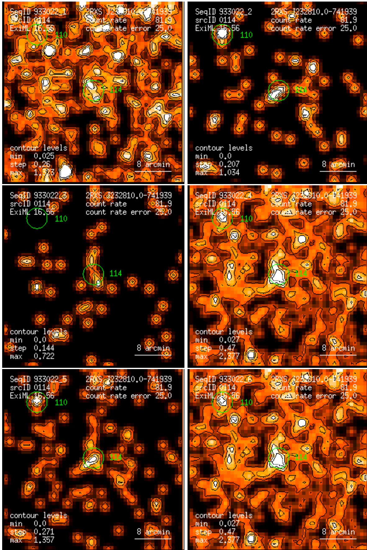
Figure 114: RASS 933022: detection 0114: band rate images, Gaussian filter: (1) PSPC channels 11 – 41, (2) 52 – 90, (3) 91 – 201, (4) 11 – 235, (5) 52 – 201, (6) 11 – 201. Broad band rates in counts/ks. Band rate contour levels in counts/ks/arcmin 2 .
