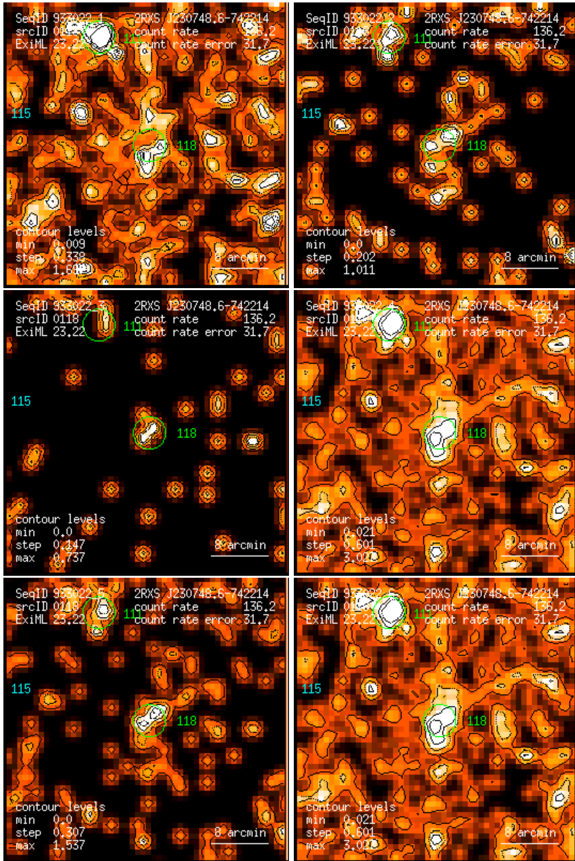
Figure 118: RASS 933022: detection 0118: band rate images, Gaussian filter: (1) PSPC channels 11 – 41, (2) 52 – 90, (3) 91 – 201, (4) 11 – 235, (5) 52 – 201, (6) 11 – 201. Broad band rates in counts/ks. Band rate contour levels in counts/ks/arcmin 2 .
