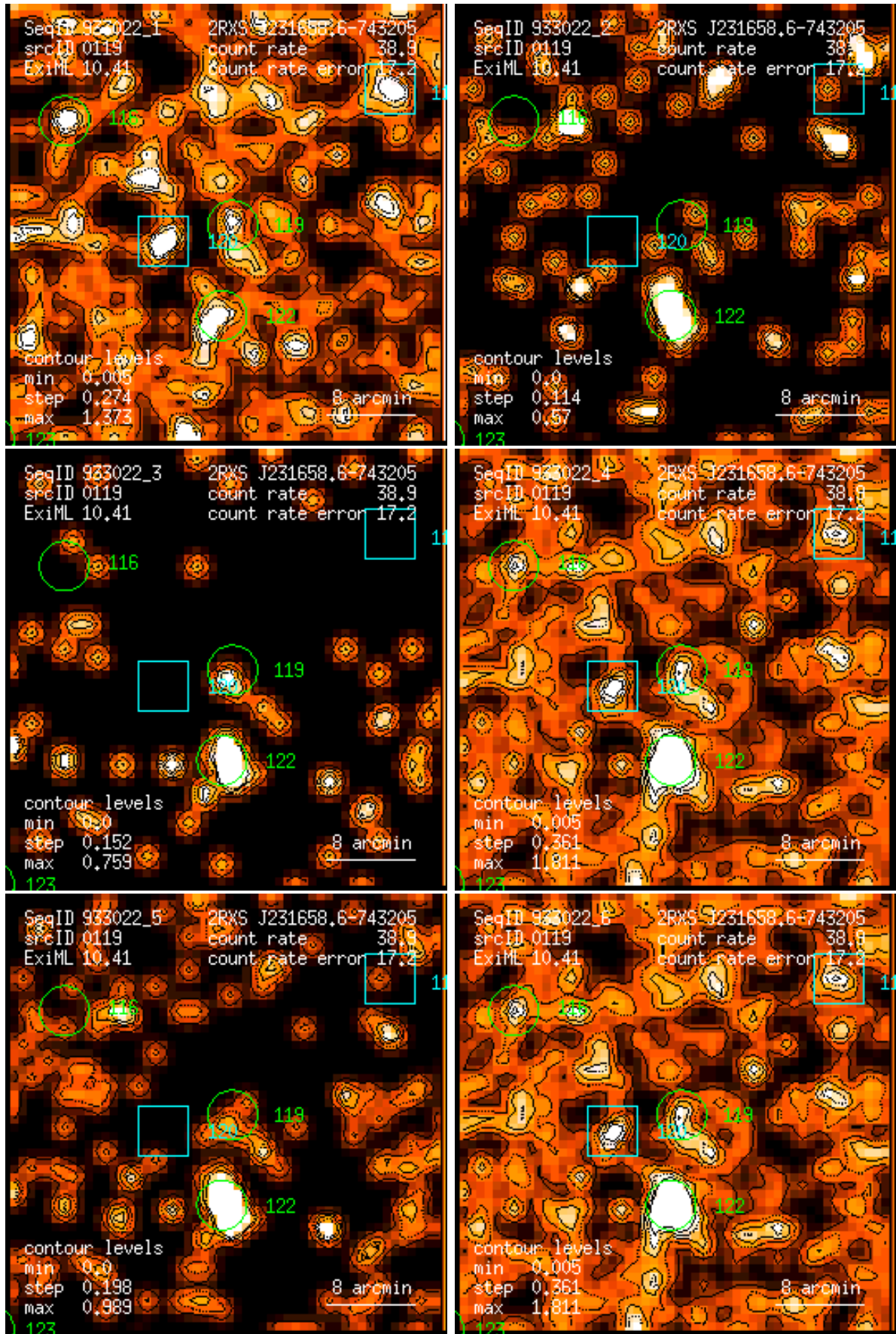
Figure 119: RASS 933022: detection 0119: band rate images, Gaussian filter: (1) PSPC channels 11 – 41, (2) 52 – 90, (3) 91 – 201, (4) 11 – 235, (5) 52 – 201, (6) 11 – 201. Broad band rates in counts/ks. Band rate contour levels in counts/ks/arcmin 2 .
