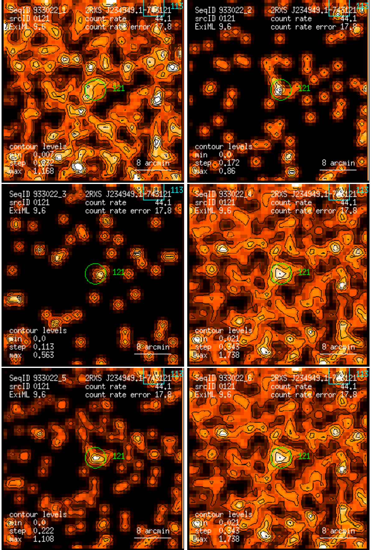
Figure 121: RASS 933022: detection 0121: band rate images, Gaussian filter: (1) PSPC channels 11 – 41, (2) 52 – 90, (3) 91 – 201, (4) 11 – 235, (5) 52 – 201, (6) 11 – 201. Broad band rates in counts/ks. Band rate contour levels in counts/ks/arcmin 2 .
