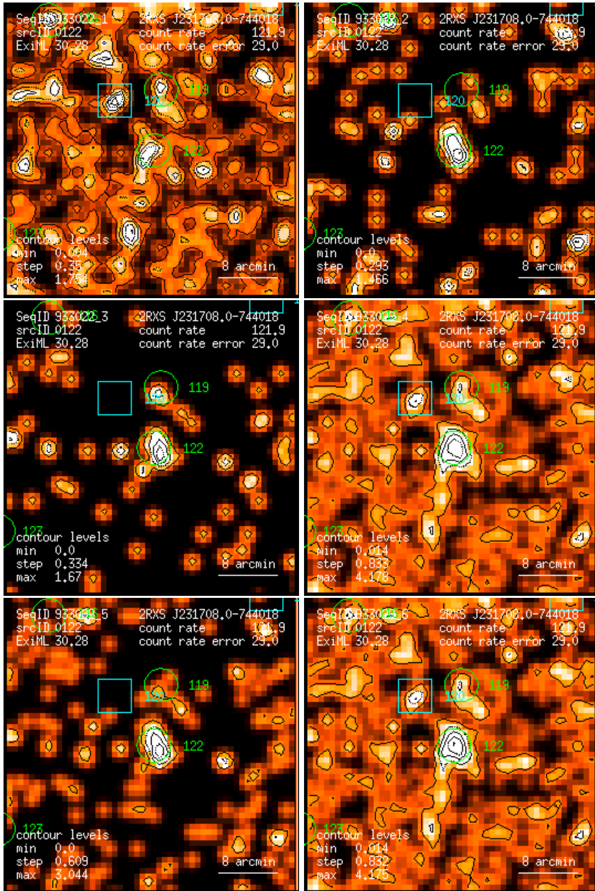
Figure 122: RASS 933022: detection 0122: band rate images, Gaussian filter: (1) PSPC channels 11 – 41, (2) 52 – 90, (3) 91 – 201, (4) 11 – 235, (5) 52 – 201, (6) 11 – 201. Broad band rates in counts/ks. Band rate contour levels in counts/ks/arcmin 2 .
