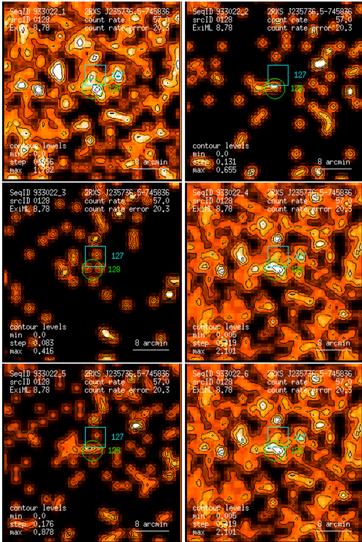
Figure 128: RASS 933022: detection 0128: band rate images, Gaussian filter: (1) PSPC channels 11 – 41, (2) 52 – 90, (3) 91 – 201, (4) 11 – 235, (5) 52 – 201, (6) 11 – 201. Broad band rates in counts/ks. Band rate contour levels in counts/ks/arcmin 2 .
