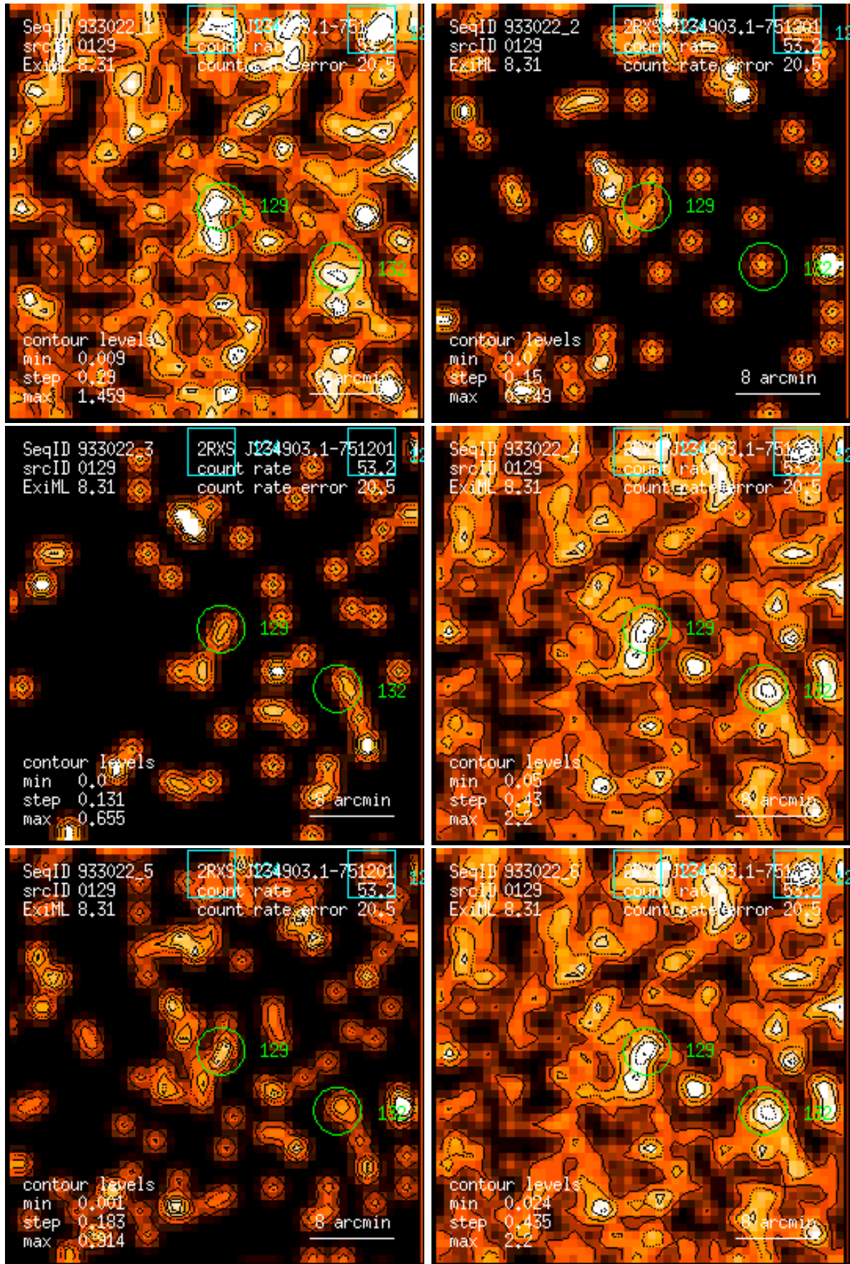
Figure 129: RASS 933022: detection 0129: band rate images, Gaussian filter: (1) PSPC channels 11 – 41, (2) 52 – 90, (3) 91 – 201, (4) 11 – 235, (5) 52 – 201, (6) 11 – 201. Broad band rates in counts/ks. Band rate contour levels in counts/ks/arcmin 2 .
