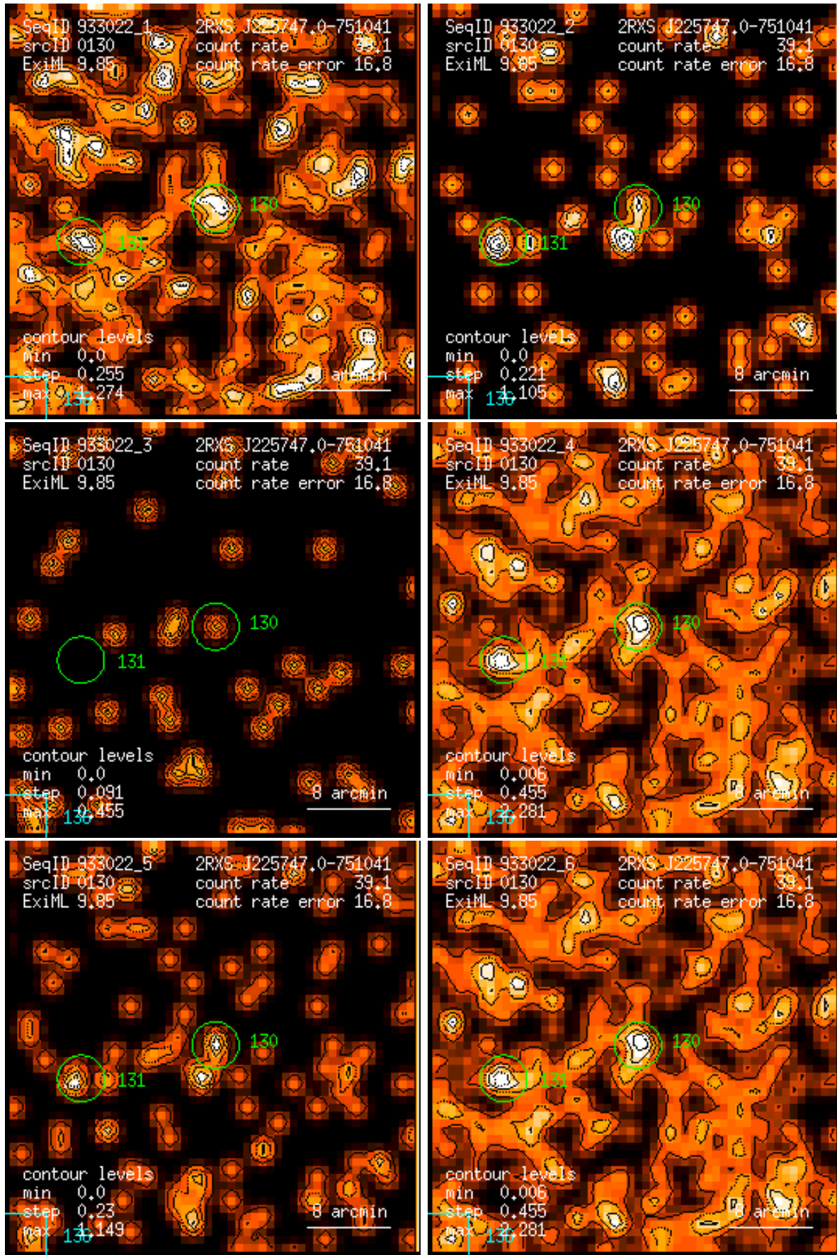
Figure 130: RASS 933022: detection 0130: band rate images, Gaussian filter: (1) PSPC channels 11 – 41, (2) 52 – 90, (3) 91 – 201, (4) 11 – 235, (5) 52 – 201, (6) 11 – 201. Broad band rates in counts/ks. Band rate contour levels in counts/ks/arcmin 2 .
