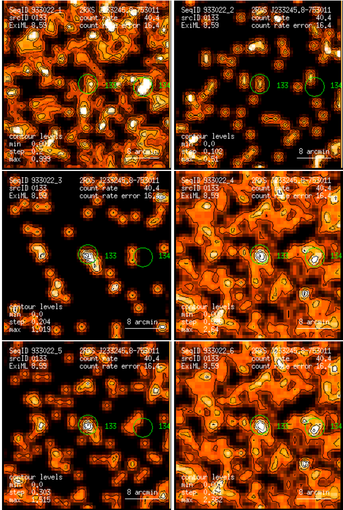
Figure 133: RASS 933022: detection 0133: band rate images, Gaussian filter: (1) PSPC channels 11 – 41, (2) 52 – 90, (3) 91 – 201, (4) 11 – 235, (5) 52 – 201, (6) 11 – 201. Broad band rates in counts/ks. Band rate contour levels in counts/ks/arcmin 2 .
