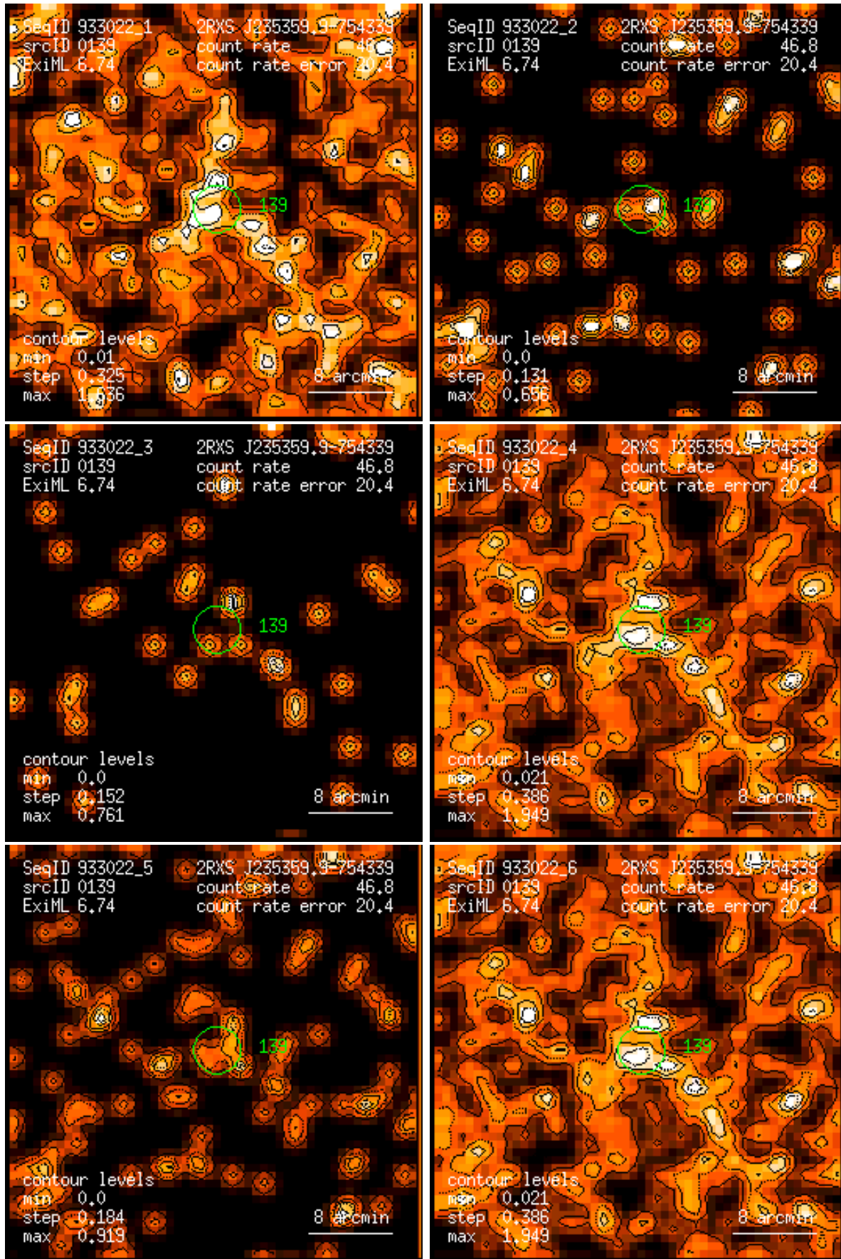
Figure 139: RASS 933022: detection 0139: band rate images, Gaussian filter: (1) PSPC channels 11 – 41, (2) 52 – 90, (3) 91 – 201, (4) 11 – 235, (5) 52 – 201, (6) 11 – 201. Broad band rates in counts/ks. Band rate contour levels in counts/ks/arcmin 2 .
