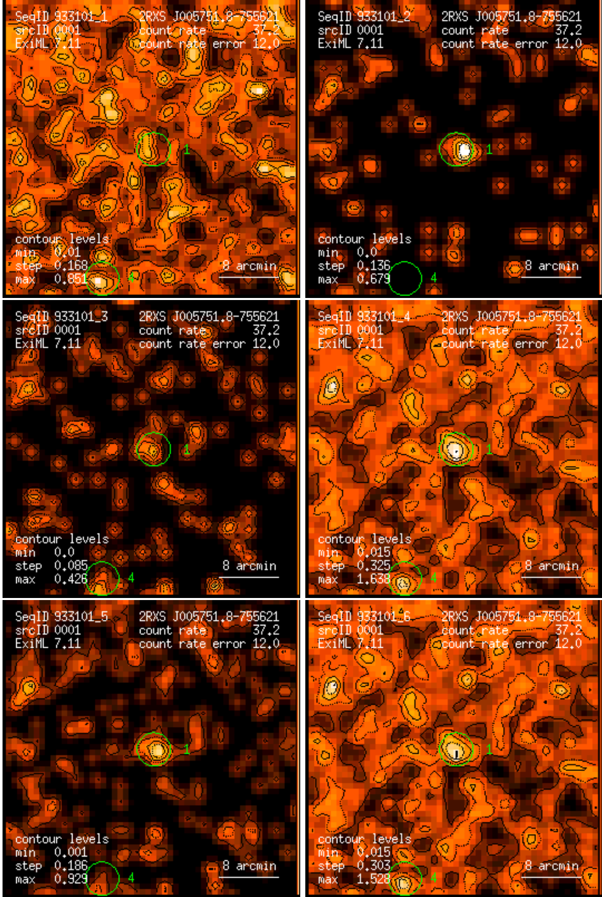
Figure 1: RASS 933101: detection 0001: band rate images, Gaussian filter: (1) PSPC channels 11 – 41, (2) 52 – 90, (3) 91 – 201, (4) 11 – 235, (5) 52 – 201, (6) 11 – 201. Broad band rates in counts/ks. Band rate contour levels in counts/ks/arcmin 2 .
