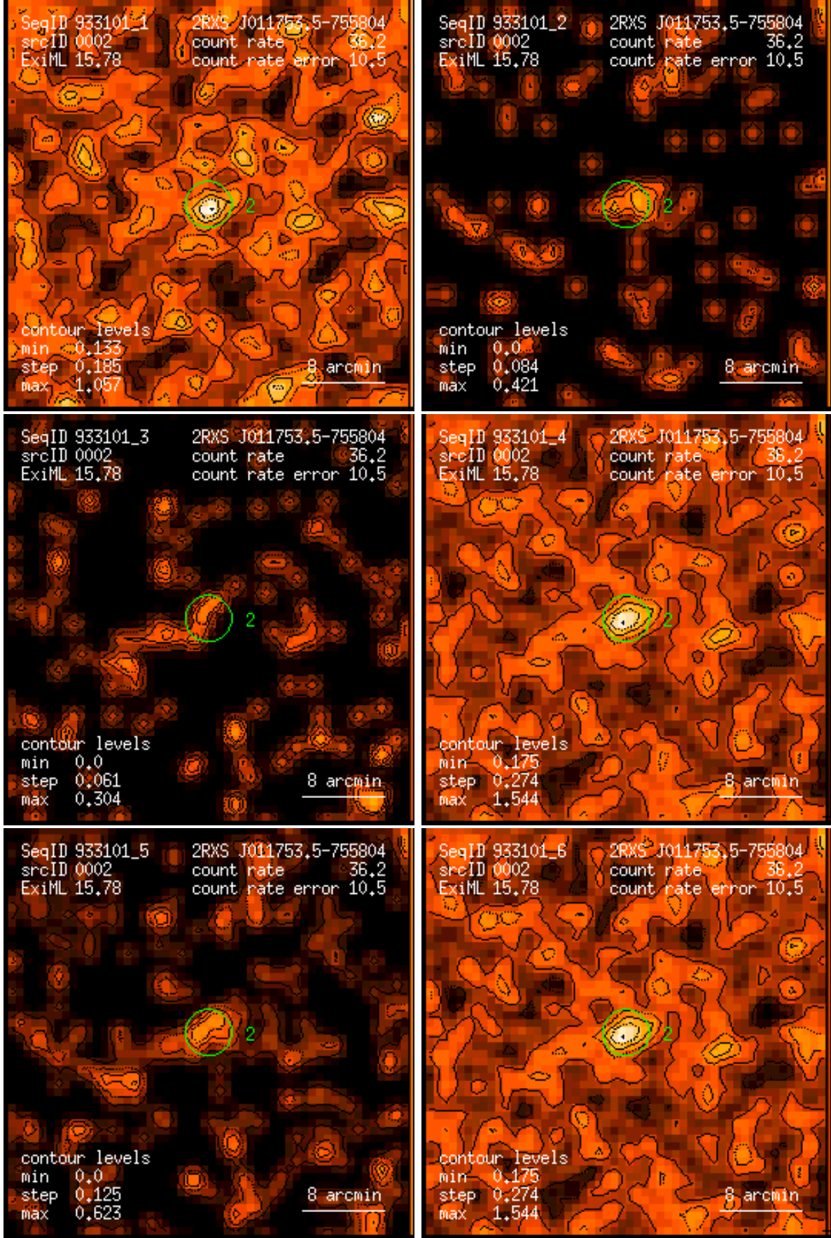
Figure 2: RASS 933101: detection 0002: band rate images, Gaussian filter: (1) PSPC channels 11 – 41, (2) 52 – 90, (3) 91 – 201, (4) 11 – 235, (5) 52 – 201, (6) 11 – 201. Broad band rates in counts/ks. Band rate contour levels in counts/ks/arcmin 2 .
