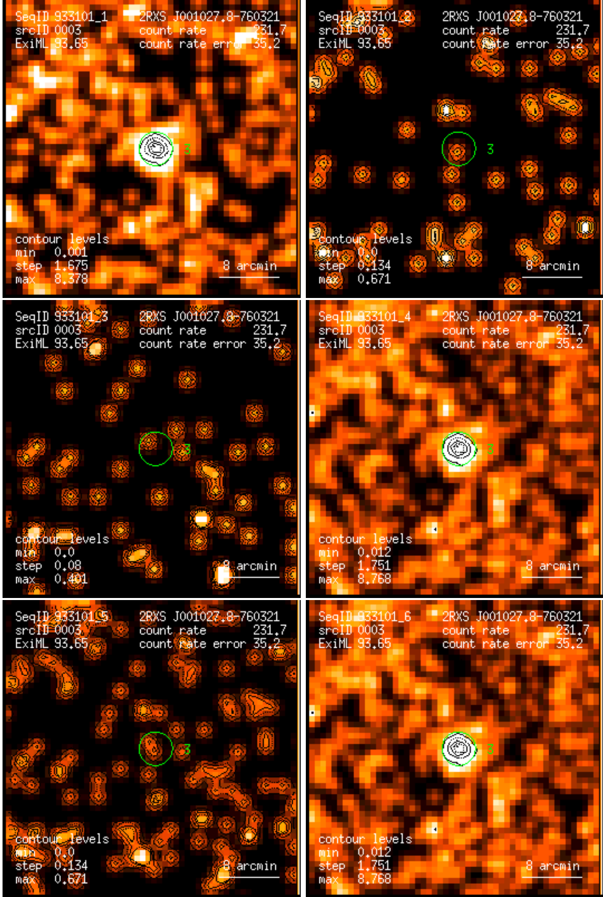
Figure 3: RASS 933101: detection 0003: band rate images, Gaussian filter: (1) PSPC channels 11 – 41, (2) 52 – 90, (3) 91 – 201, (4) 11 – 235, (5) 52 – 201, (6) 11 – 201. Broad band rates in counts/ks. Band rate contour levels in counts/ks/arcmin 2 .
