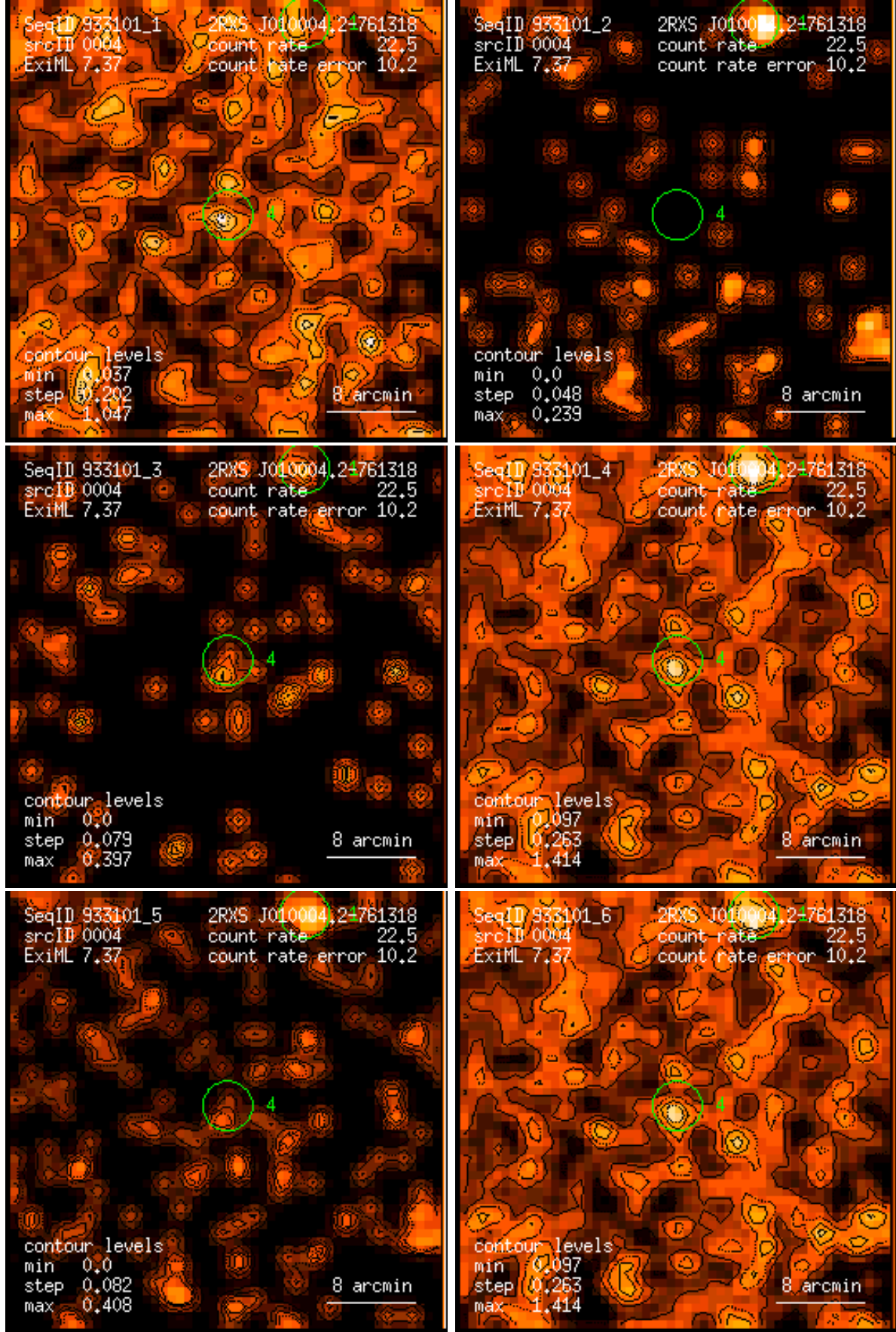
Figure 4: RASS 933101: detection 0004: band rate images, Gaussian filter: (1) PSPC channels 11 – 41, (2) 52 – 90, (3) 91 – 201, (4) 11 – 235, (5) 52 – 201, (6) 11 – 201. Broad band rates in counts/ks. Band rate contour levels in counts/ks/arcmin 2 .
