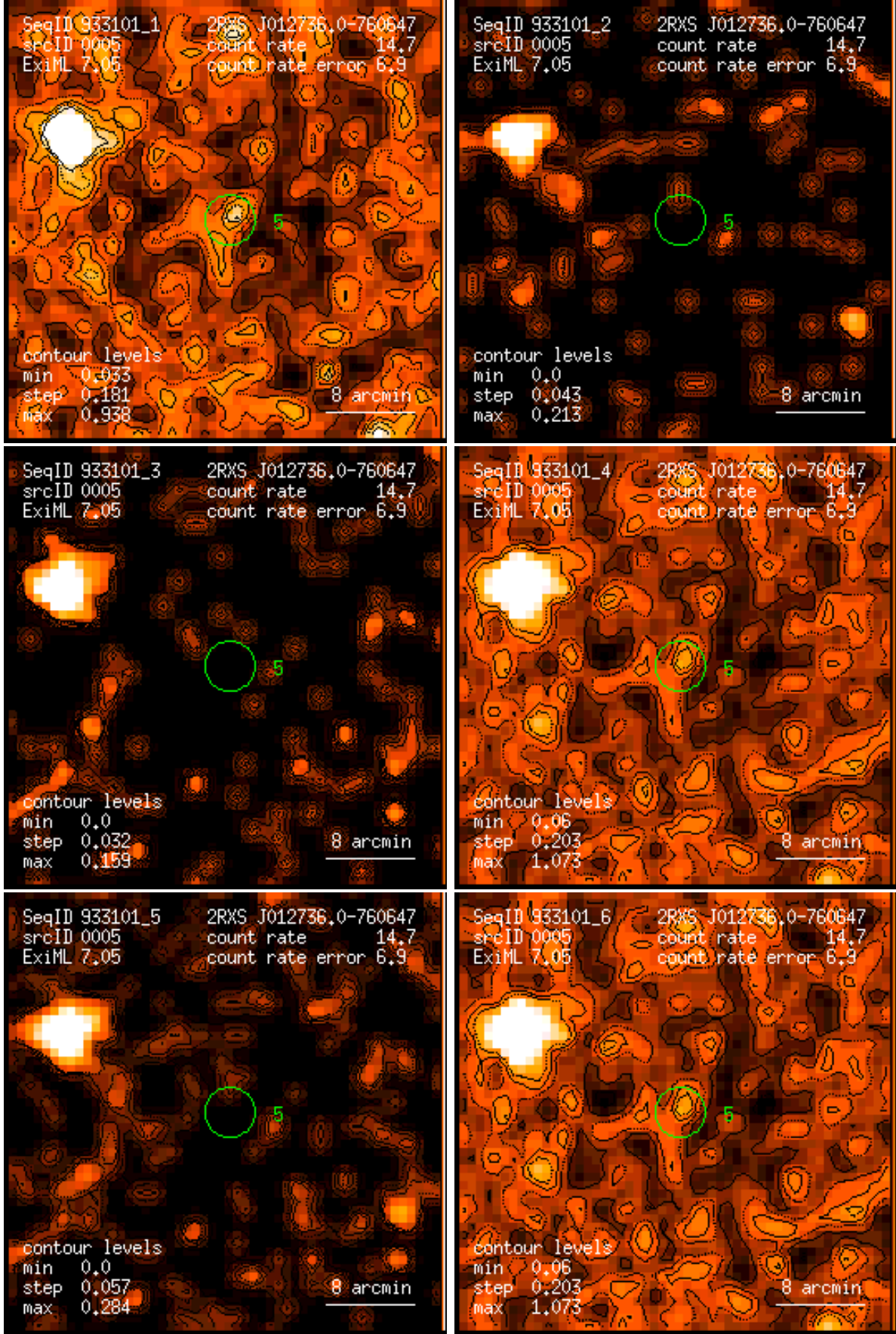
Figure 5: RASS 933101: detection 0005: band rate images, Gaussian filter: (1) PSPC channels 11 – 41, (2) 52 – 90, (3) 91 – 201, (4) 11 – 235, (5) 52 – 201, (6) 11 – 201. Broad band rates in counts/ks. Band rate contour levels in counts/ks/arcmin 2 .
