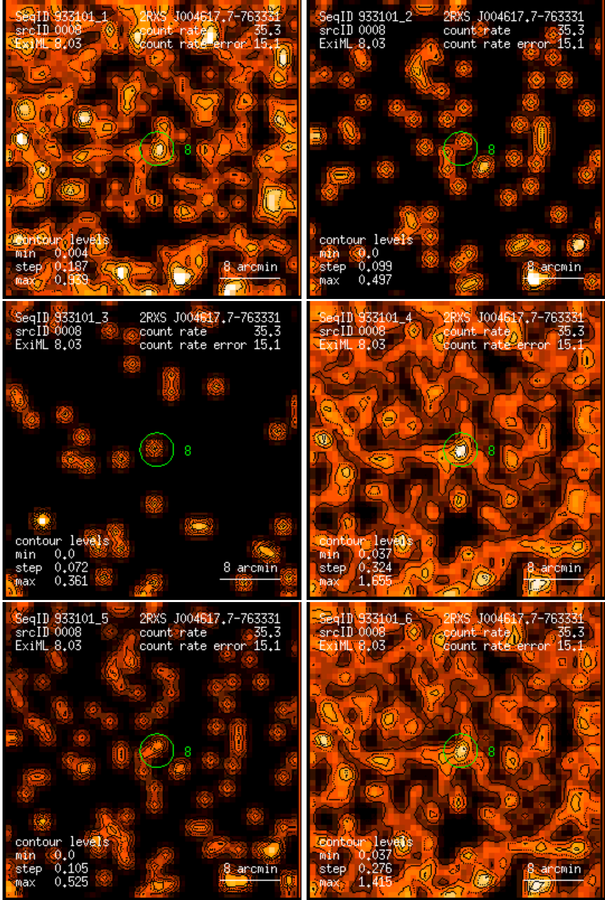
Figure 8: RASS 933101: detection 0008: band rate images, Gaussian filter: (1) PSPC channels 11 – 41, (2) 52 – 90, (3) 91 – 201, (4) 11 – 235, (5) 52 – 201, (6) 11 – 201. Broad band rates in counts/ks. Band rate contour levels in counts/ks/arcmin 2 .
