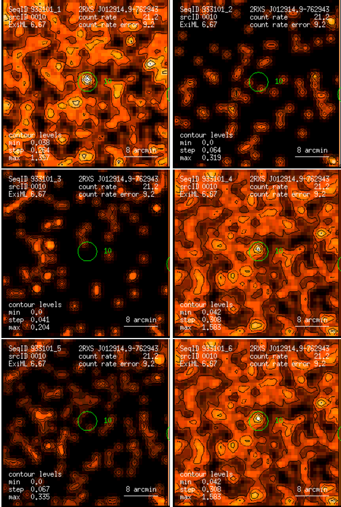
Figure 10: RASS 933101: detection 0010: band rate images, Gaussian filter: (1) PSPC channels 11 – 41, (2) 52 – 90, (3) 91 – 201, (4) 11 – 235, (5) 52 – 201, (6) 11 – 201. Broad band rates in counts/ks. Band rate contour levels in counts/ks/arcmin 2 .
