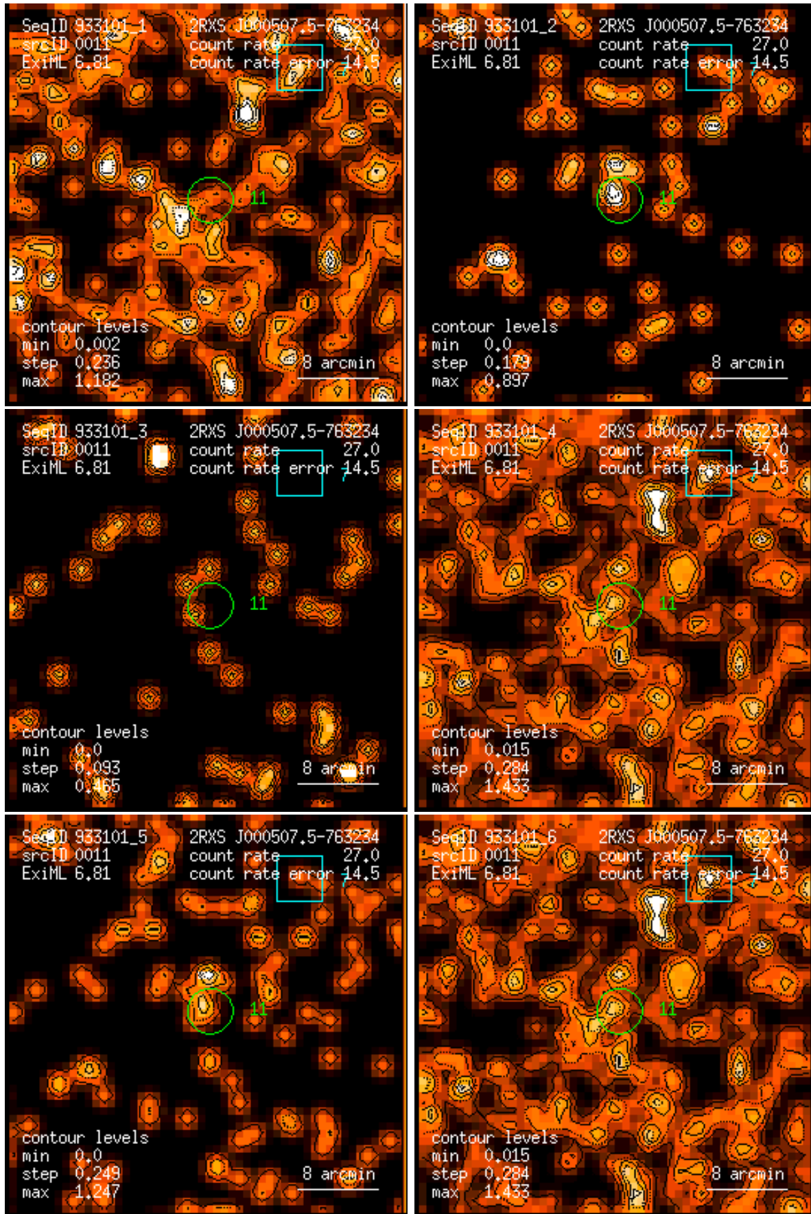
Figure 11: RASS 933101: detection 0011: band rate images, Gaussian filter: (1) PSPC channels 11 – 41, (2) 52 – 90, (3) 91 – 201, (4) 11 – 235, (5) 52 – 201, (6) 11 – 201. Broad band rates in counts/ks. Band rate contour levels in counts/ks/arcmin 2 .
